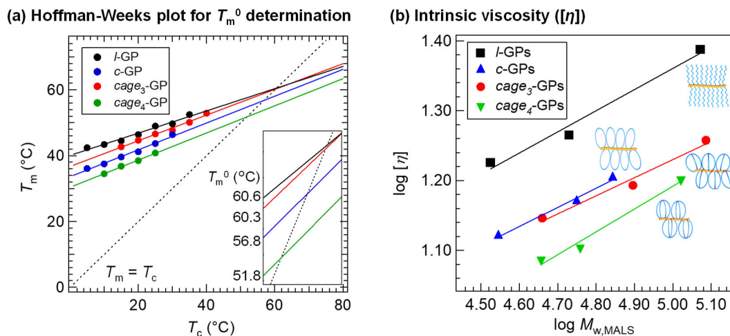
Figure 4. Structure-property relationships of topological GPCLs and their counterparts. (a) Hoffman-Weeks plot of GPCLs. The inset contains a magnification of the plot around the point of intersection, which represents the T_m^0 value of each GPCL. (b) Double-logarithmic plots of M_{w,MALS} versus [\eta] for l -GPCLs (black), c -GPCLs (blue), cage 3 -GPCLs (red), and cage 4 -GPCLs (green) (in THF).
