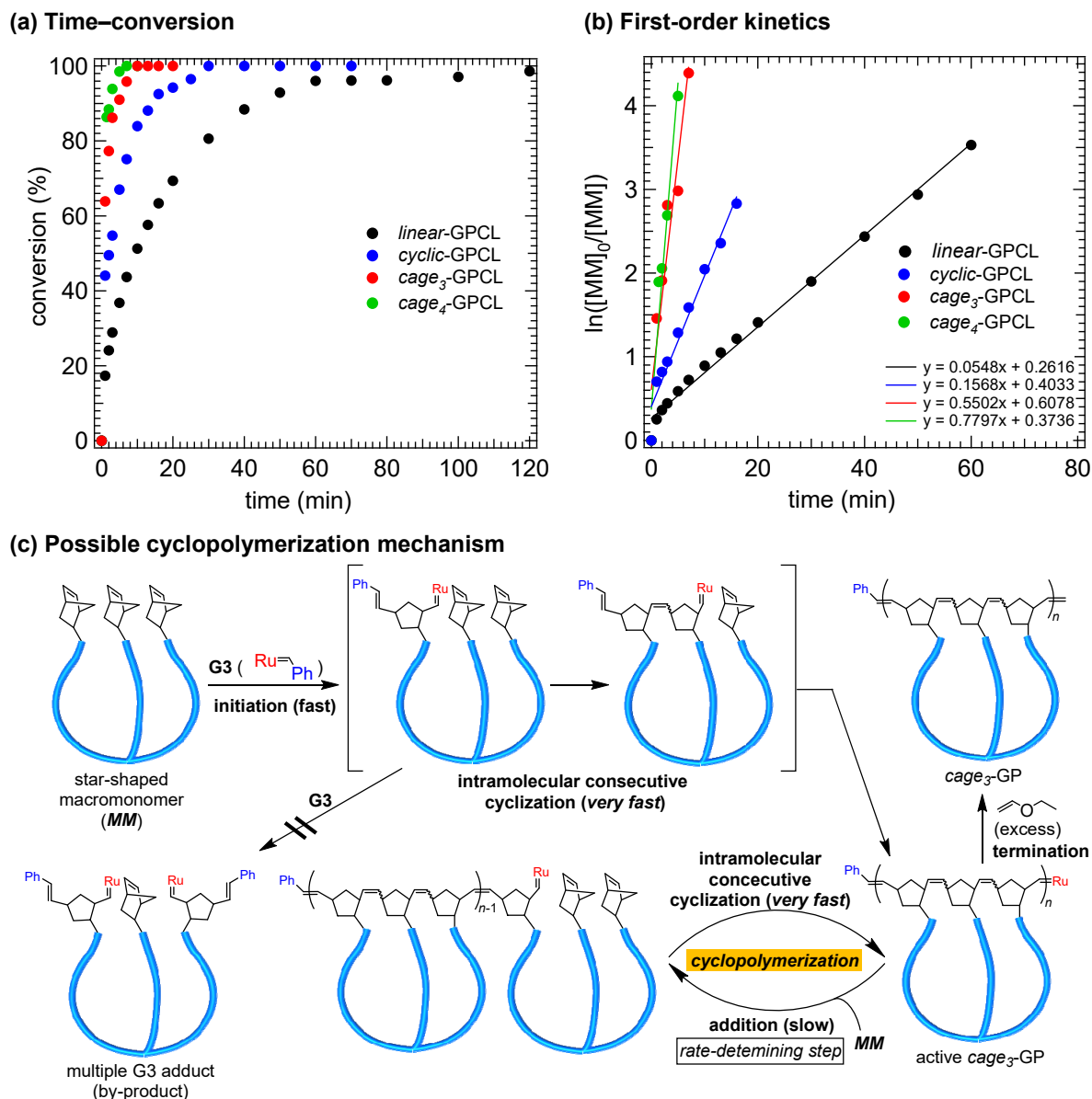
Figure 3. (a,b) Kinetic analyses of the (cyclo)polymerizations of PCL-NB, NB-PCL-NB, s -(PCL-NB) 3 , and s -(PCL-NB) 4 ([PCL-NB] 0 /[G3] 0 = 15/1; [NB-PCL-NB] 0 /[G3] 0 = 7.5/1; [ s -(PCL-NB) 3 ] 0 /[G3] 0 = 5/1; [ s -(PCL-NB) 4 ] 0 /[G3] 0 = 3.75/1; [MM] 0 = 0.2 mM). (c) Proposed mechanism for the cyclopolymerization of three-armed star-shaped macromonomers to produce a well-defined cage 3 -GPCL under a diluted condition.
