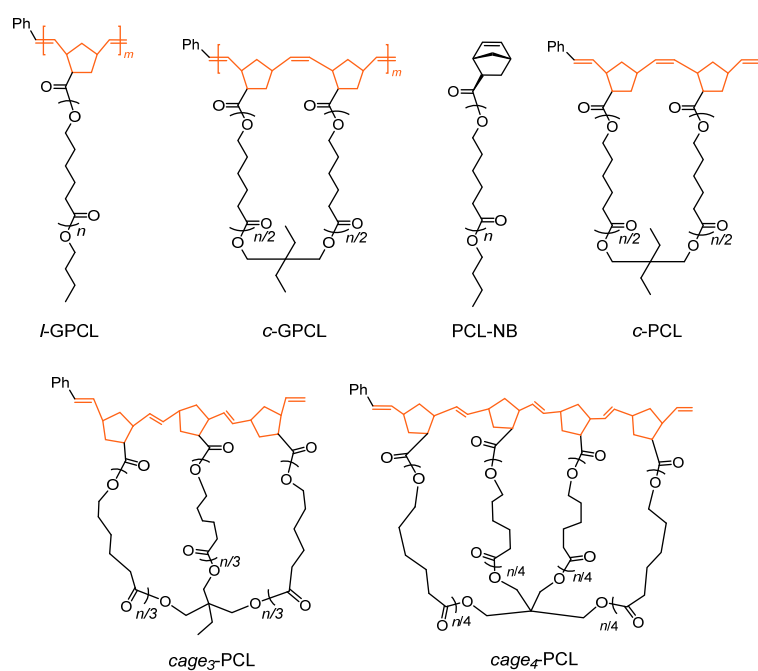
Chart 1. List of topological counterparts used for systematic characterization. Linear and cyclic GPCLs ( l -GPCL and c -GPCL) and monomeric PCLs (PCL-NB, c -PCL, cage 3 -PCL, and cage 4 -PCL)
