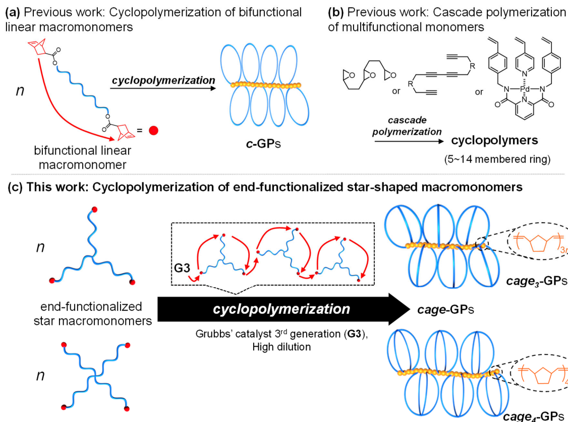
Figure 1. Schematic of cyclopolymerization strategies for constructing architecturally unique polymers. (a) Cyclopolymerization of linear bifunctional macromonomers to produce cyclic GPs ( c -GPs). (b) Cascade polymerization of multifunctional monomers to produce corresponding cyclopolymers having small rings. (c) Cyclopolymerization of norbornenyl-end-functionalized star-shaped macromonomers to synthesize cage -GPs.
