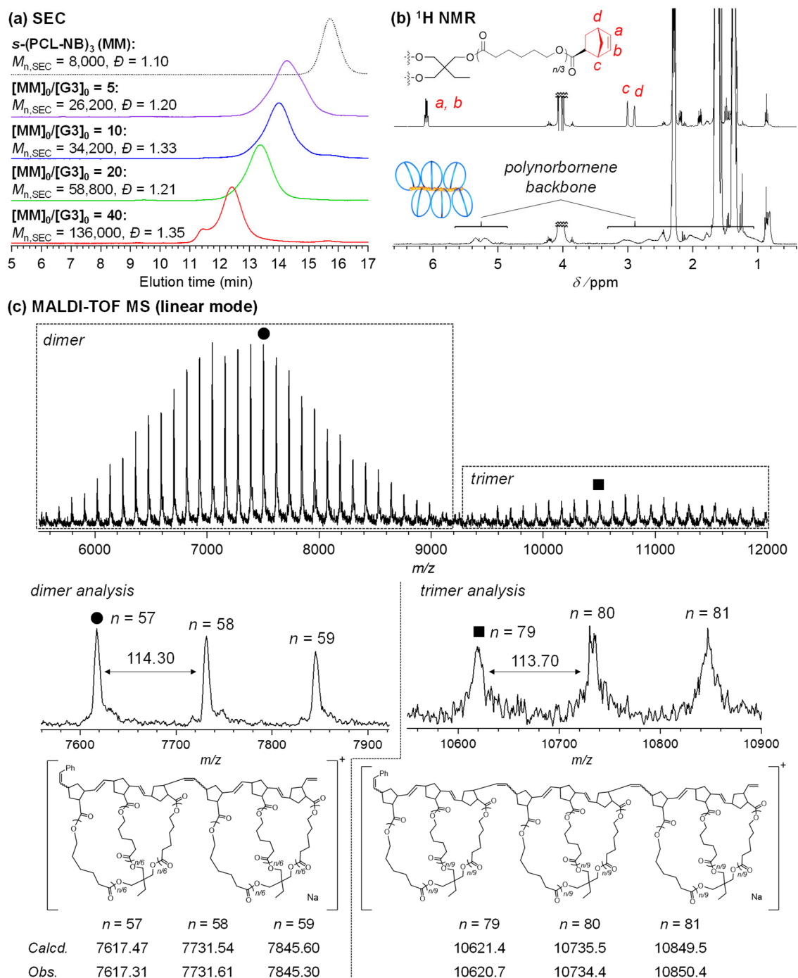
Figure 2. Structural analysis of graft polymers containing three-armed cage-shaped PCL side-chains ( cage 3 -GPCLs) prepared by cyclopolymerization using G3. (a) SEC traces of the three-armed star-shaped macromonomer (MM, namely s -(PCL-NB) 3 ; M_{n,NMR} = 5,200 \text{ g mol}^{-1} , M_{n,SEC} = 8,000 \text{ g mol}^{-1} , \bar{D} = 1.10 ; dotted line) and the cage 3 -GPCLs obtained at [MM] 0 /[G3] 0 = 5 (purple), 10 (blue), 20 (green), and 40 (red) in THF. The shoulder peak that appeared in the SEC traces of the product obtained at [MM] 0 /[G3] 0 = 40 is due to the exclusion limit of the column (see Figure S4). (b) 1 H NMR spectra of s -(PCL-NB) 3 (upper) and cage 3 -GPCL prepared at [MM] 0 /[G3] 0 = 5 (lower) in CDCl 3 (400 MHz). (c)
