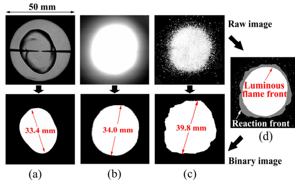
Fig. 2 Images processing; (a) ammonia/oxygen/nitrogen flame; (b) luminous flame in co-combustion; (c) OH radical image in co-combustion; (d) OH radical image processing
