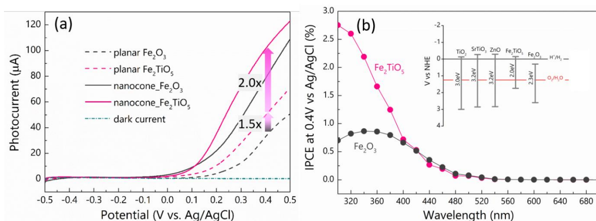
Fig. 4 (a) Anodic photocurrent from 50 nm Fe 2 O 3 and Fe 2 TiO 5 thin films on planar ITO substrates (dashed lines) and ITO nanocones (solid lines). (b) The dependence of the anodic photocurrent from the planar thin films on the wavelength of the incident light. The inset shows the energy diagram of several common oxide materials for photocatalysis.
