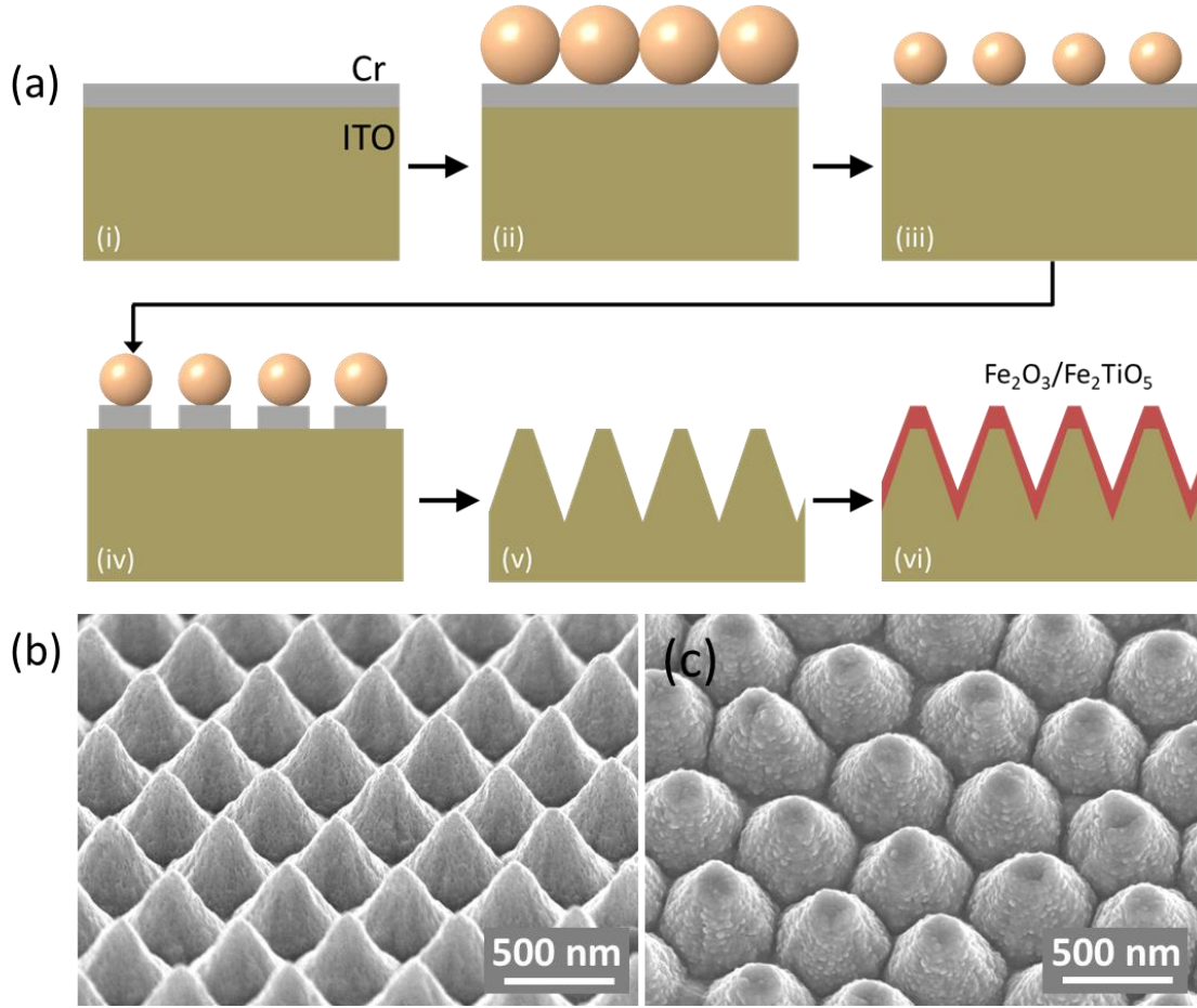
Fig. 2. (a) Illustration (not to scale) of the fabrication process of the ITO/Fe 2 O 3 (ITO/Fe 2 TiO 5 ) nanocones. (i) 30 nm Cr layer was deposited onto the ITO films; (ii) colloidal self-assembly of PS nanospheres; (iii) Shrinking the size of the nanospheres with O 2 plasma etching; (iv) etching of the Cr layer using the etched PS spheres as masks; (v) Creation of ITO nanocones using Cr disks as masks; (vi) deposition of Fe 2 O 3 (Fe 2 TiO 5 ) onto the ITO nanocones. (b) SEM image of the ITO nanocones created with 500 nm PS spheres. (c) SEM image of ITO/Fe 2 O 3 hybrid nanocones created with 500 nm PS spheres.
