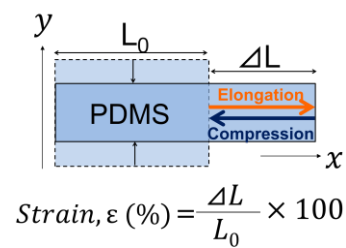
Figure 4.24: Definition of stretch strain. Stretching strain, \epsilon , where L_0 is initial length of substrate (15 mm) and \Delta L is the change of length (7.8 mm) after applying strain.
