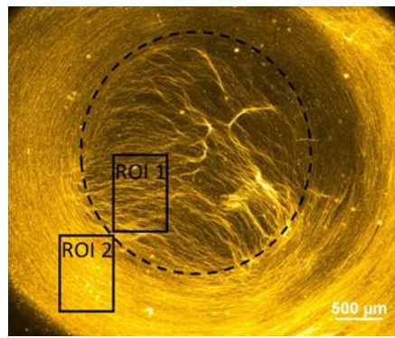
Figure 4.12: Selection of ROI to calculate nematic order parameter with time two region separated through an imaginary boundary. Scale bar: 500 \mu\text{m} .
