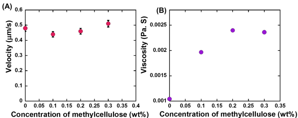
Figure 2.12: Effect of methyl cellulose concentration on the (A) velocity of gliding microtubules and (B) buffer viscosity.
