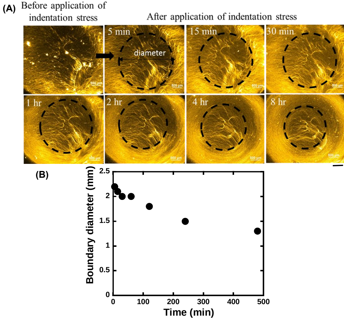
Figure 4.10: (A) Fluorescence images of collectively moving microtubules showing decrease of inner boundary of the vortex pattern (dotted line), and (B) change of diameter of inner boundary with time. Scale bar: 500 \mu\text{m} .
