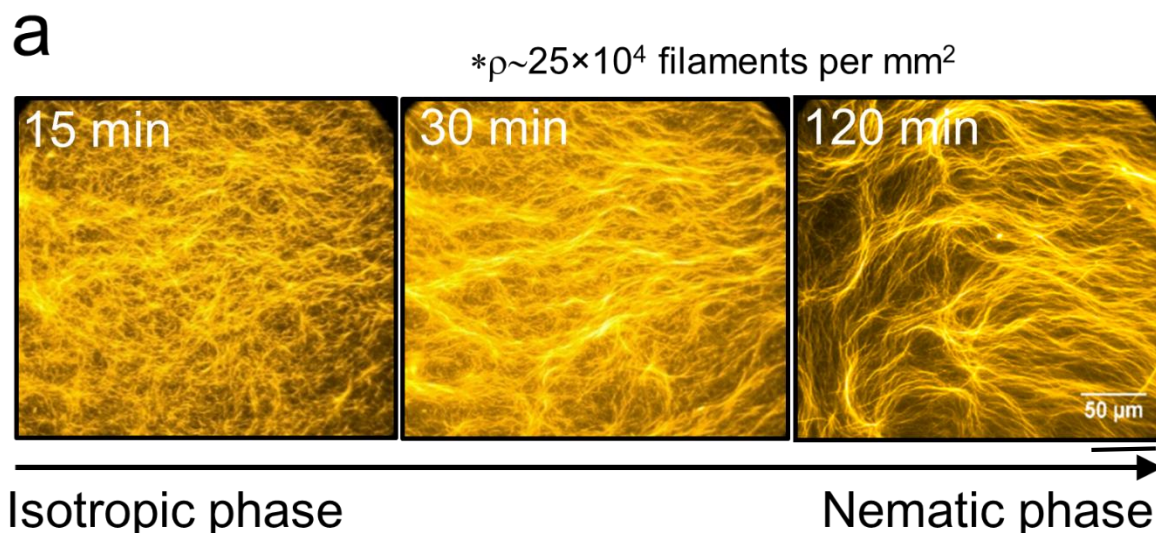
Figure 3.1: Time-lapse fluorescence images showing emergence of stream pattern by the collective motion of GTP-microtubules. Scale bar: 50 \mu\text{m} .
