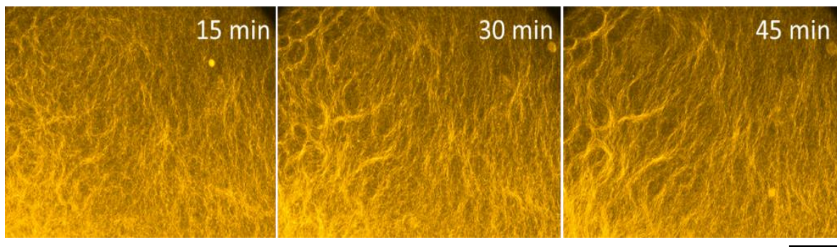
Figure 4.5: Time-lapse fluorescence image of microtubules showing emergence of collective motion on PDMS substrate. Scale bar: 100 \mu\text{m} .
