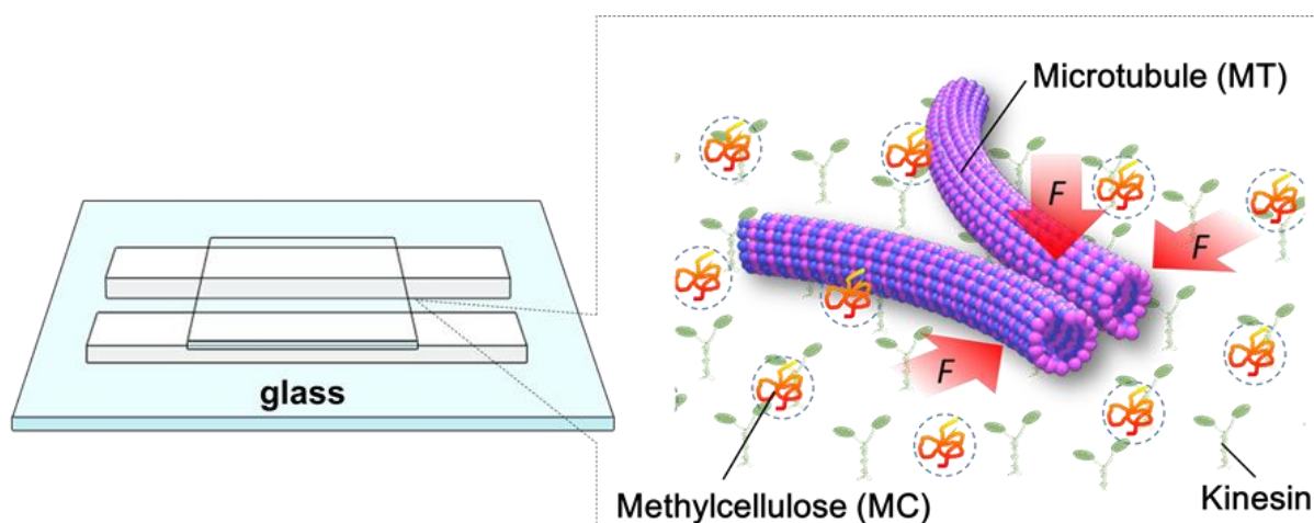
Figure 2.1: Schematic diagram of the experimental set up and illustration of the in vitro motility assay used to investigate collective motion of microtubules driven by kinesins.
