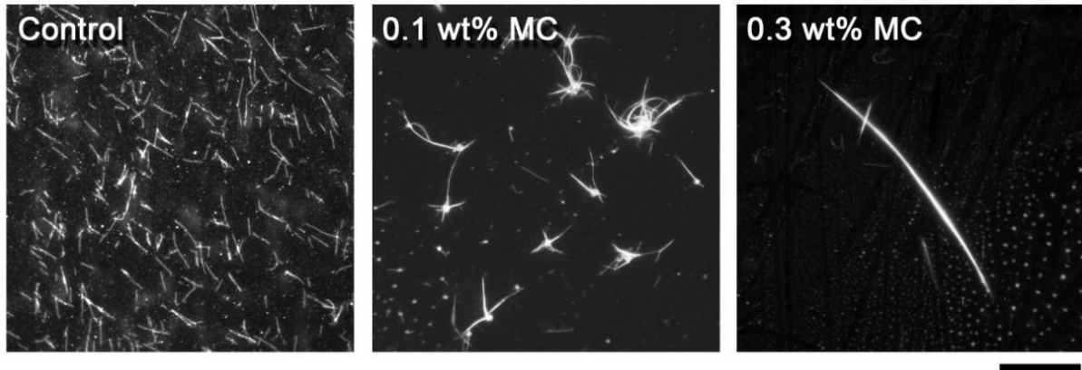
Figure 2.2: Depletion force induced bundle formation of microtubules. Fluorescence microscopic images of microtubules, which were suspended in solution (left) without methyl cellulose and (middle, right) with methyl cellulose. Scale bar: 10 \mu\text{m} .
