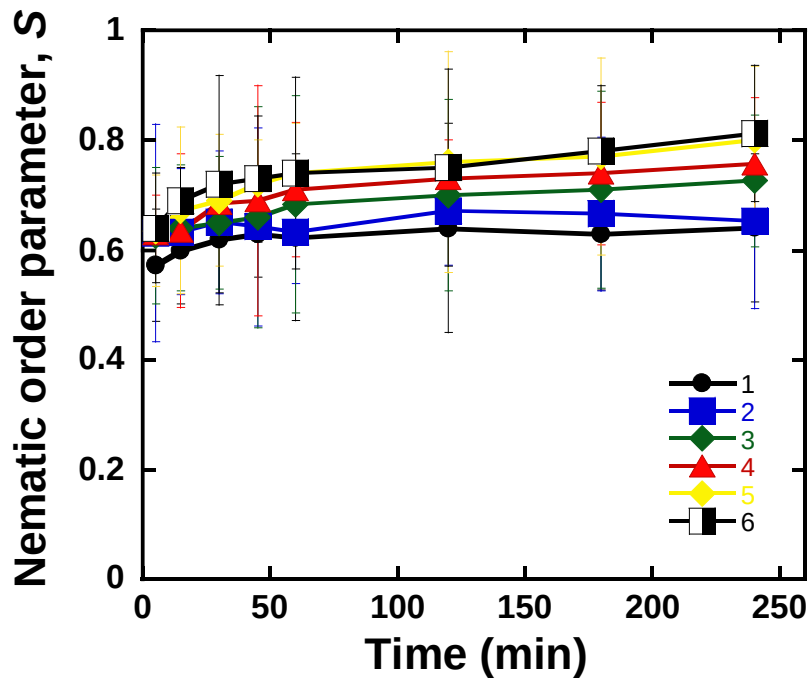
Figure 4.8: Change of nematic order parameter of microtubules with time. Here 1, 2, 3, 4, 5, 6, 7 indicates the corresponding ROI shown in Figure 4.7.
