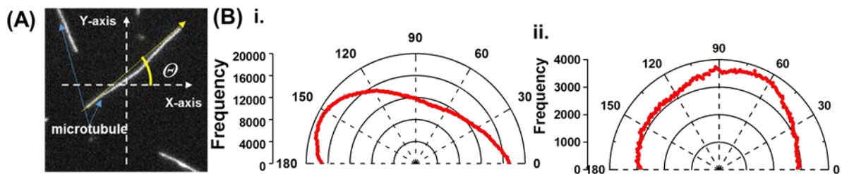
Figure 2.5: (A) Schematic representation of analysis of microtubule orientation angle \Theta . Yellow arrow represents moving direction of microtubules. As shown here, the orientation angle was measured with respect to the X-axis. Scale bar: 5 \mu\text{m} . (B) Circular histogram of orientation angle of microtubules in absence of methyl cellulose at (i) 0 min and (ii) 120 min
