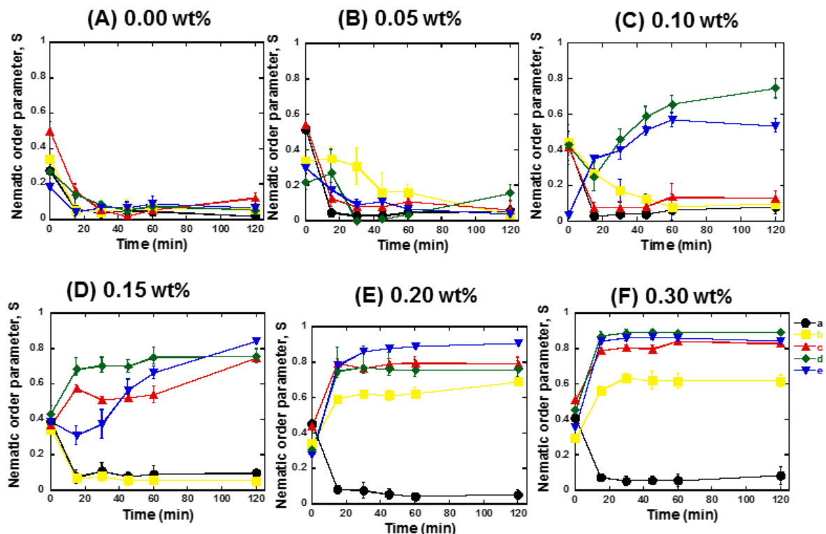
Figure 2.9: Change of the orientation of microtubules with time at different concentrations of methyl cellulose and microtubule. In each case the concentration of methyl cellulose is mentioned above the figure (from 0.0 to 0.3 wt%). In the figures the lines a, b, c, d, and e represent order parameter for 1.0, 3.0, 5.0, 10.0, and 15.0 \mu M microtubules respectively
