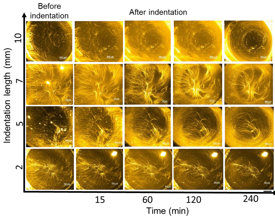
Figure 4.11: Fluorescence images of collectively moving microtubules before and after application of indentation stress with different indentation length of 2, 5, 7, and 10 mm. Scale bar: 500 μm.
