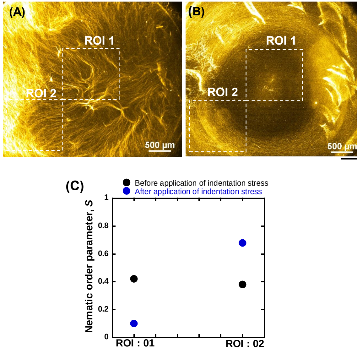
Figure 4.21: Fluorescence images of orientation of microtubules (A) before and (B) after 1 hour of application of indentation stress. (C) The corresponding order parameters in ROI: 1 and ROI: 2; before and after indentation. Scale bar: 500 \mu\text{m} .
