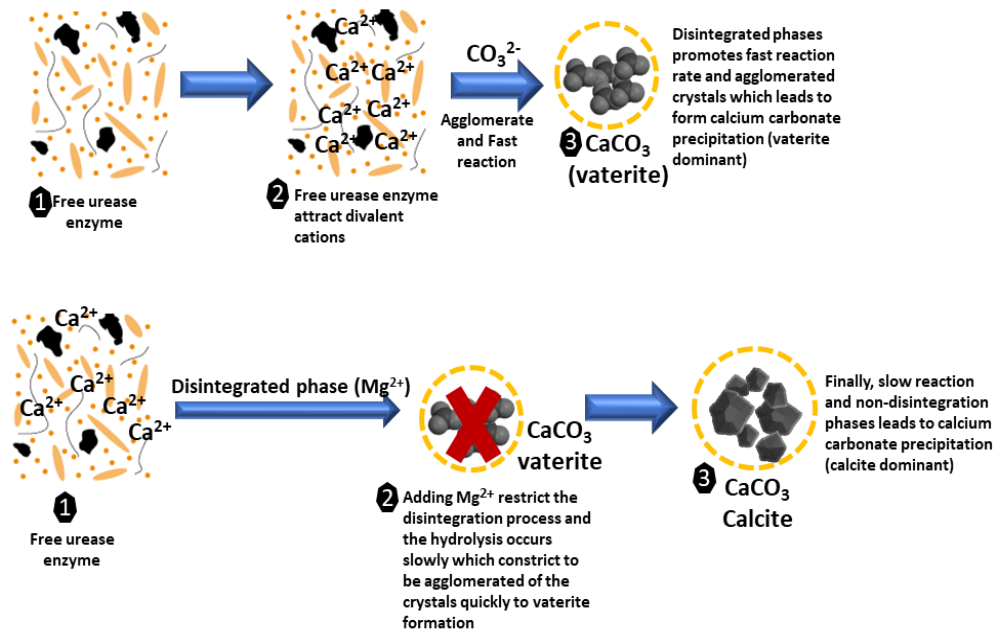
Figure 4. 14: Schematic illustration of the \text{CaCO}_3 formation mechanism (calcite and vaterite) in contract with \text{Mg}^{2+}/\text{Ca}^{2+} ratios.
