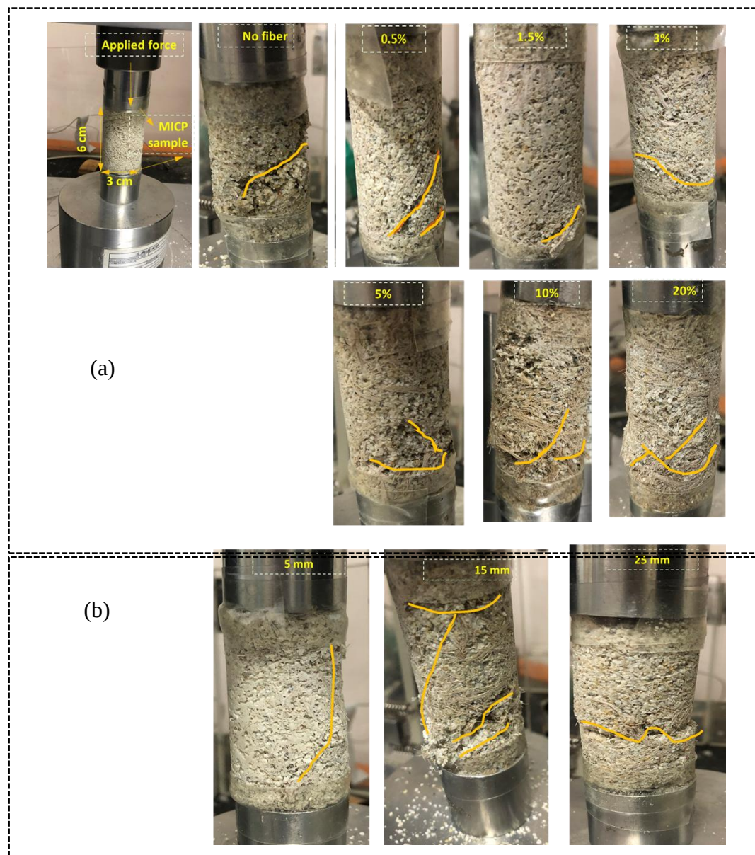
Figure 5. 18: Effect Failure behavior of the MICP treated sample by addition of jute fiber: (a) fiber content (b) fiber length.
