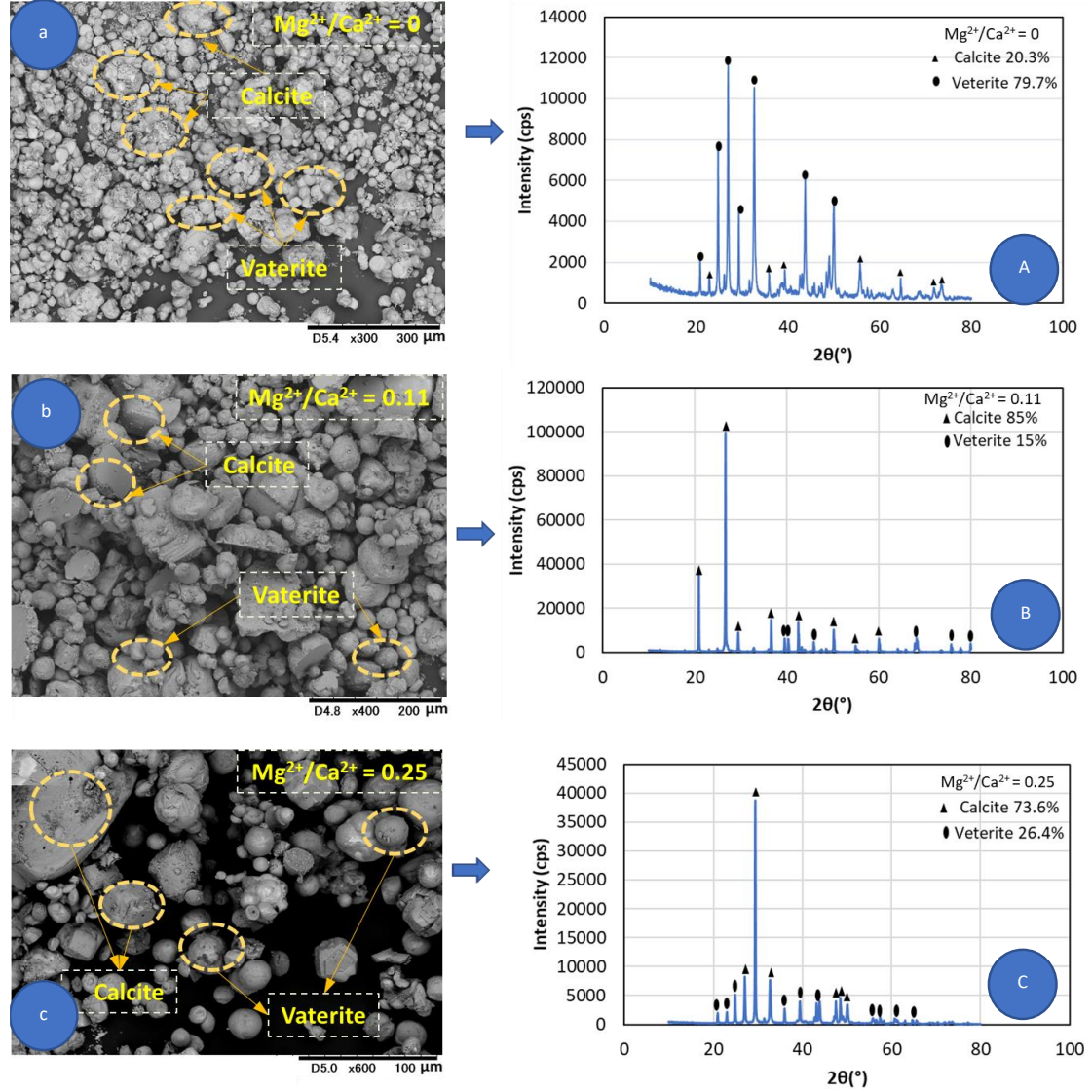
Figure 4. 12: SEM images of the precipitated \text{CaCO}_3 crystals with different \text{Mg}^{2+}/\text{Ca}^{2+} ratios (a–c) and their subsequent XRD analysis to confirm the polymorph of the crystals (A–C).
