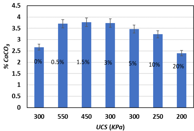
Figure 6. 4: Average (%) \text{CaCO}_3 of the biocemented sand after EICP treatment by addition of jute fiber.
