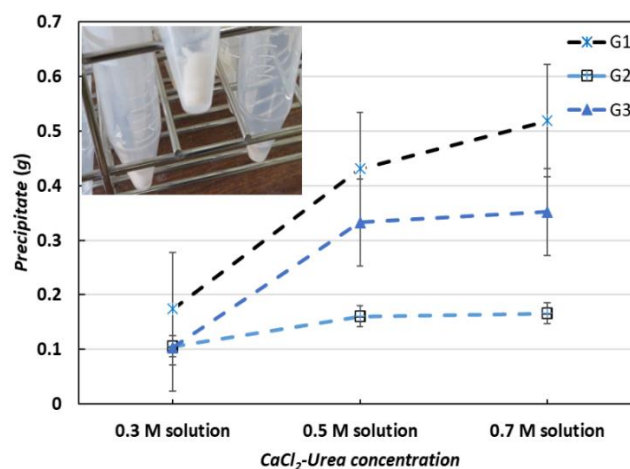
Figure 3. 15: Crystal's precipitation pattern.
