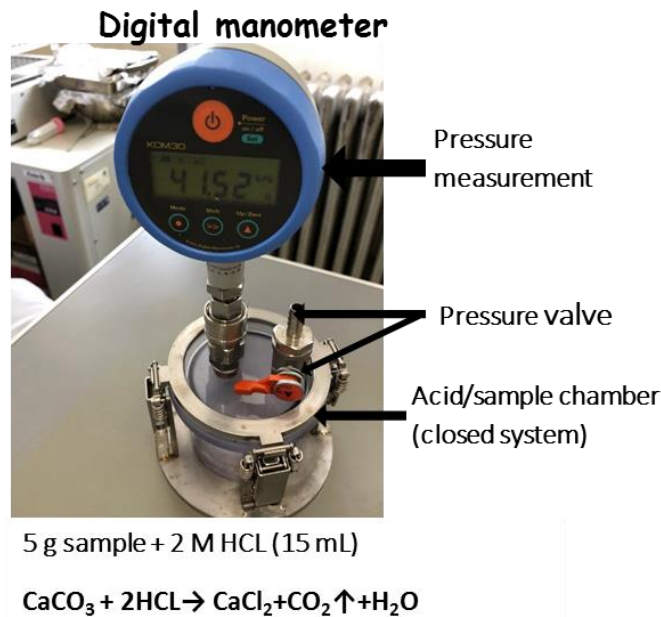
Figure 3. 7: Digital manometer set up for measuring CaCO 3 content.
