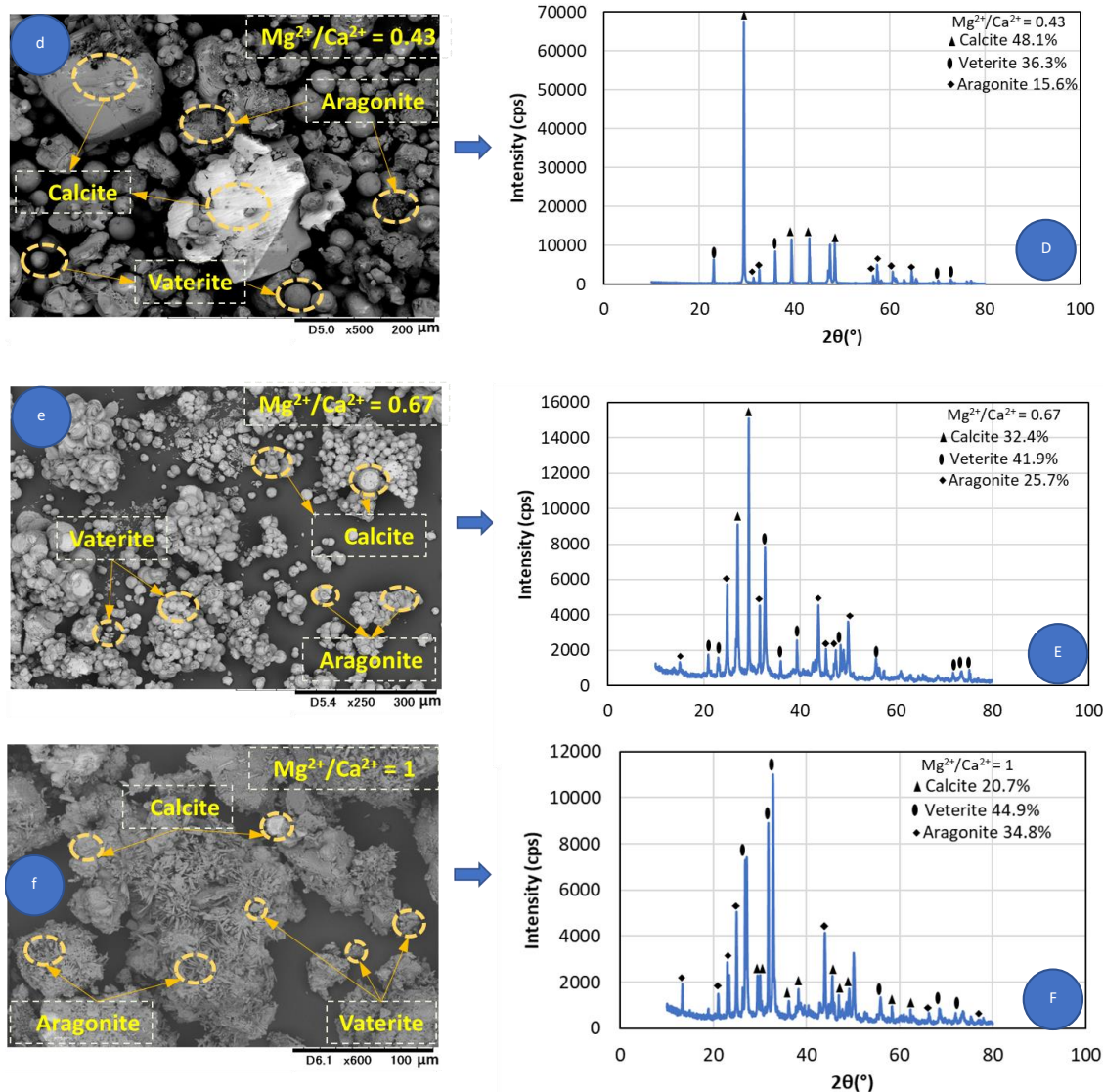
Figure 4. 13: SEM images of the precipitated \text{CaCO}_3 crystals with different \text{Mg}^{2+}/\text{Ca}^{2+} ratios (d–f) and their subsequent XRD analysis to confirm the polymorph of the crystals (D–F).
