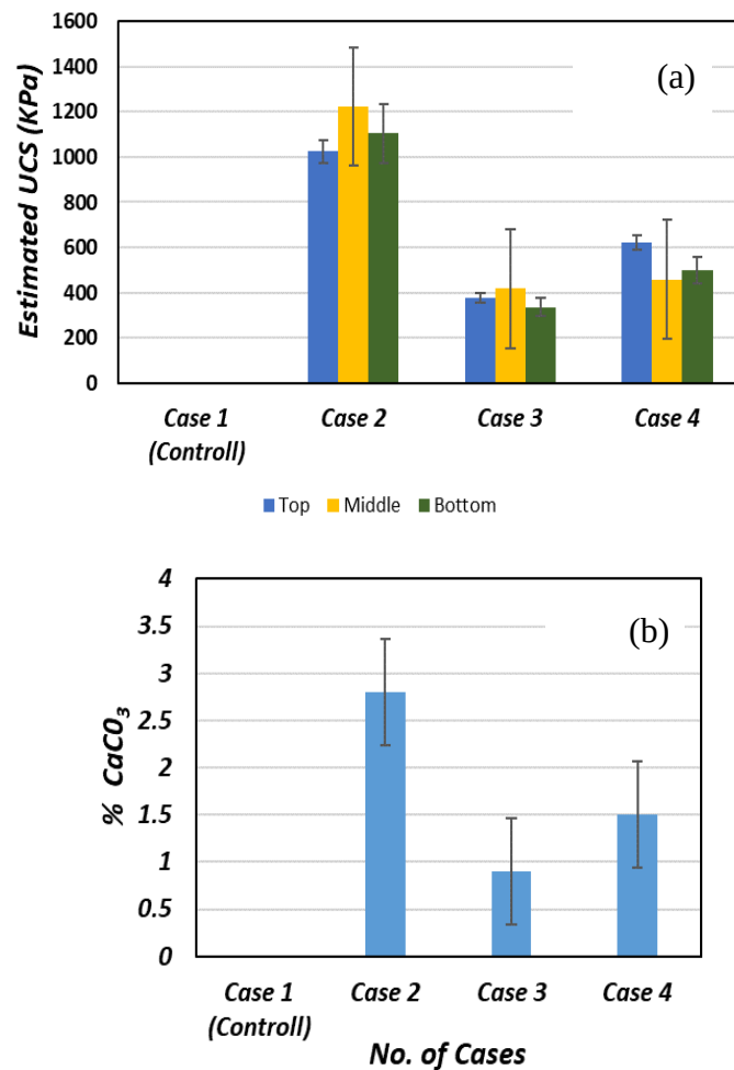
Figure 3. 17: (a) variation of UCS and (b) calcium carbonate content of G1.
