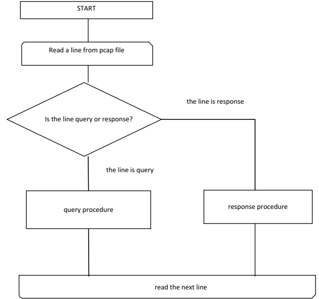
Figure 2: Flow chart of NS_DB operations
