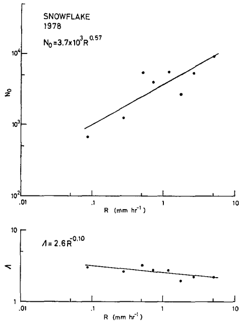
Fig. 3 Size distributions for snowflakes observed in 1978, in terms of N_0 and \lambda versus precipitation rate R (for equation N_D = N_0 \exp(-\lambda D) ).
