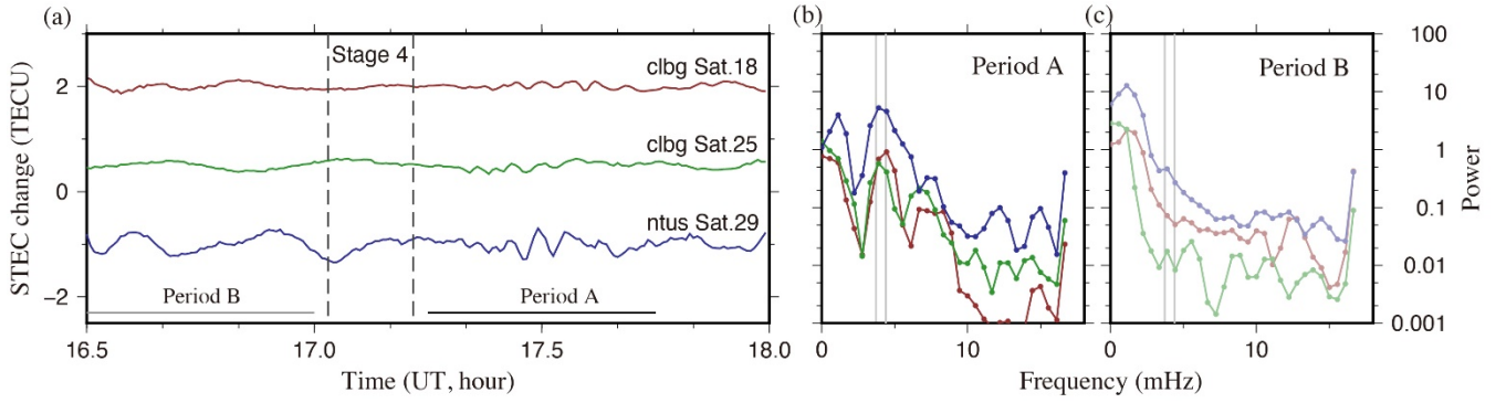
Figure 4 (a) The high-pass filtered STEC time-series at clbg (GPS Sat. 18 and 25) and ntus (GPS Sat. 29) show monochromatic oscillation lasting ~20 minutes shortly after the stage 4 of the Merapi eruption. Two gray horizontal lines show time windows (Period A 17:15-17:45 UT, Period B 16:30-17:00) used for the spectral analyses of the two periods. (b) Period A shows peaks around 4 mHz, close to the two atmospheric resonance frequencies 3.7 and 4.4 mHz (two vertical lines in light gray), but (c) Period B does not show such peaks.
