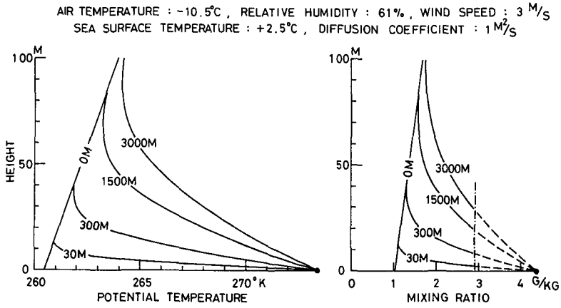
Fig. 5 Change of vertical distributions of potential temperature and mixing ratio with downwind distance. Meteorological variables are indicated in figure.
