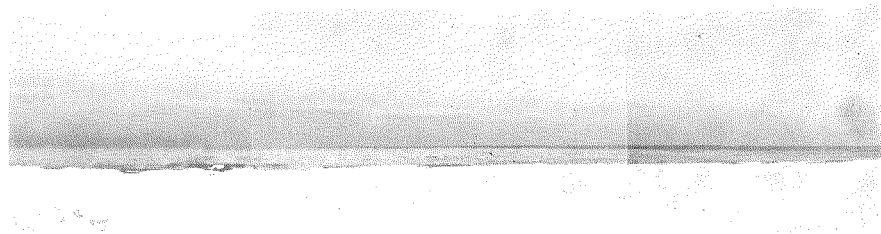
Fig. 3 Steam fog at Ishikari shore, 0828 24th January 1972.
