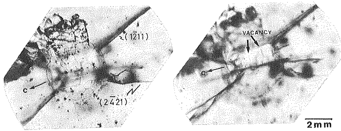
Fig. 4 Cracks created at prism plane by falling of a steel ball. Left: Surface of specimen. Right: Layer at a depth of 10 \mu\text{m} from its surface. Cracks parallel to (2\bar{4}21) and vacancies created at crack shown by arrows.
