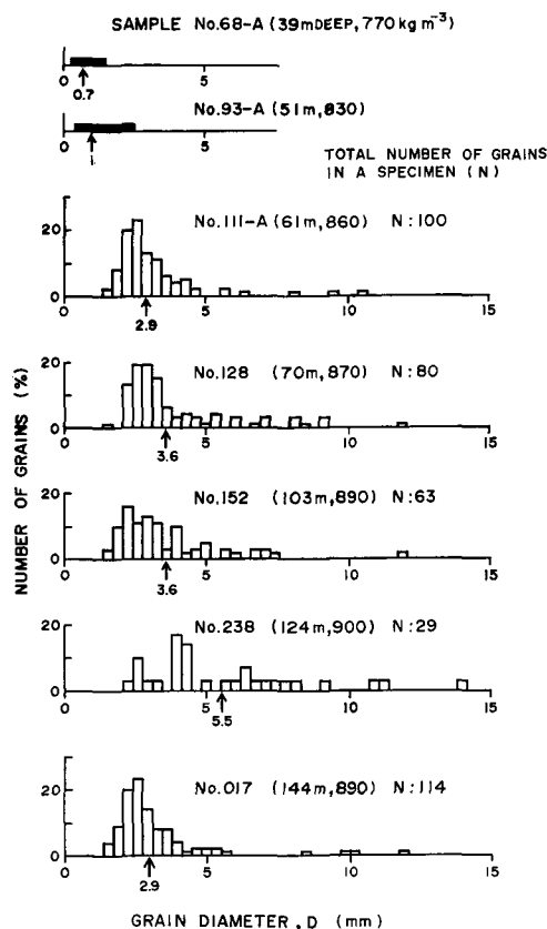
Fig. 2 Grain diameter distribution of ice specimens. Grading: 0.34 \leq D < 0.68 mm, \dots (D: diameter). The weighted mean diameter is indicated with an arrow. Sample number, depth and density are also shown above each distribution histogram.
