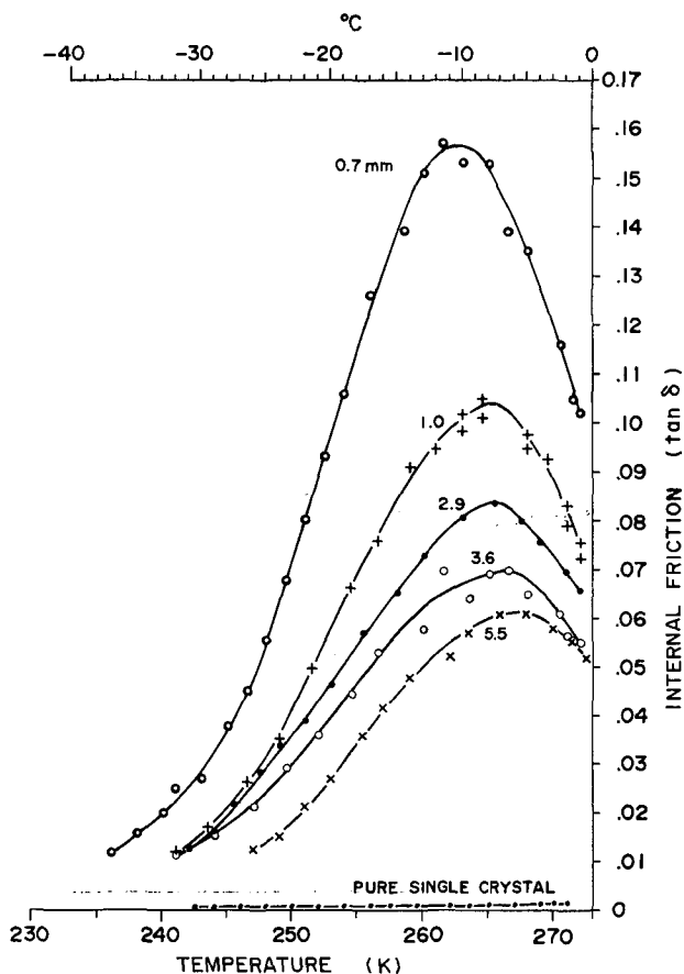
Fig. 4 Effect of grain size on the grain-boundary peak of the Antarctic Mizuho ice. The weighted mean diameter is 0.7 mm (sample No. 68-A, density 770 \text{ kg m}^{-3} ), 1.0 (No. 93-A, 830), 2.9 (No. 111-A, 860), 3.6 (No. 128, 870) and 5.5 (No. 238, 900) from top to bottom, respectively as shown in the figure.
