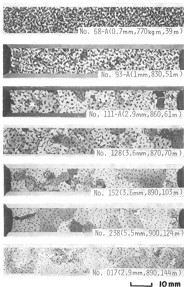
Fig. 1 Thin ice sections used for the internal friction measurement. Black ends of the specimen show top and bottom holders. Figures at the right-hand side indicate sample number, mean grain diameter, density and depth.
