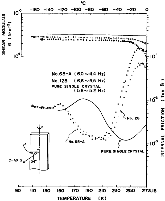
Fig. 3 Internal friction and shear modulus as a function of temperature. Samples No. 68-A and No. 128. Figures in parentheses indicate frequency in Hz from low temperature (for example, 6.0 Hz in No. 68-A) to high temperature (4.4 Hz). An internal friction curve for a pure single crystal ice is also shown. Angle between the C-axis and the torsional axis of the single crystal is shown at the left-bottom of the figure.
