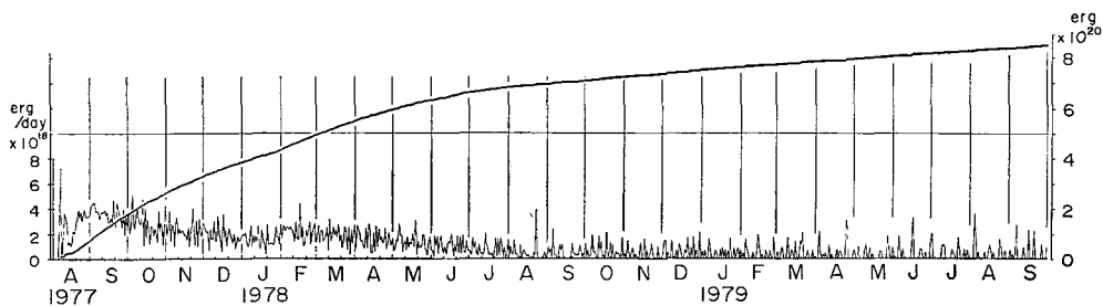
Fig. 4 Daily discharge of seismic energy and the accumulated sum.
