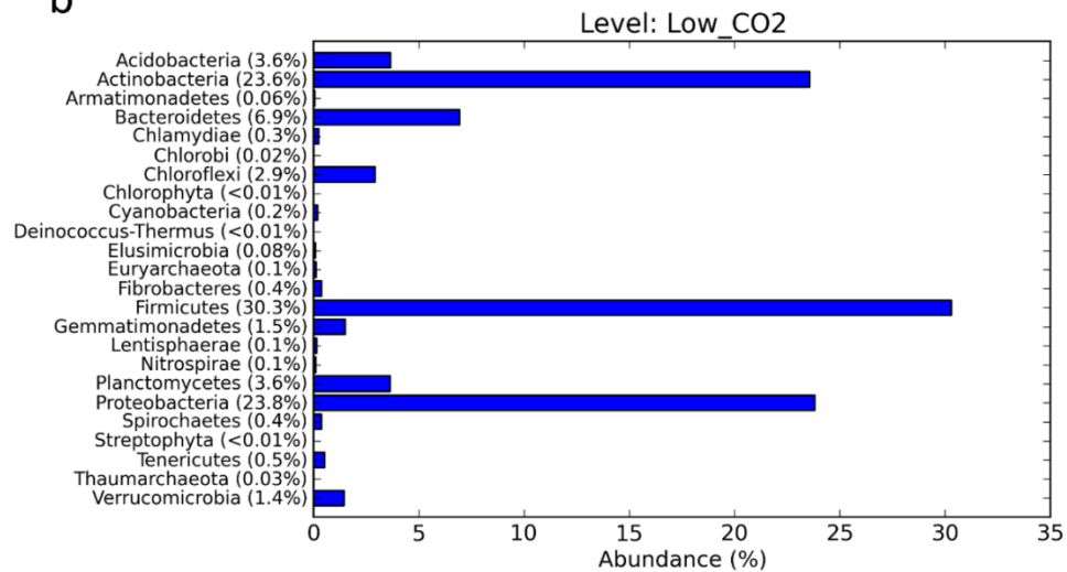
Figure 5-S2i. Unique OTUs that are specific to the a) high CO 2 and b) low CO 2 emissions under dung applied treatments.
