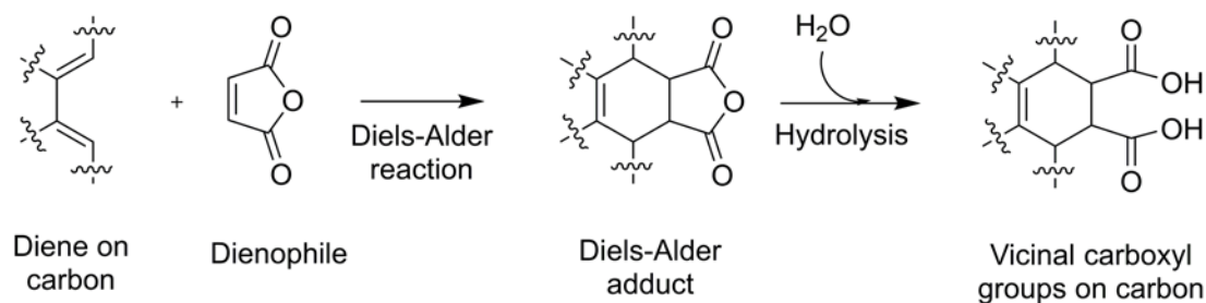
Scheme 1: Strategy for incorporation of vicinal carboxyl groups on carbon surface by Diels-Alder reaction.
