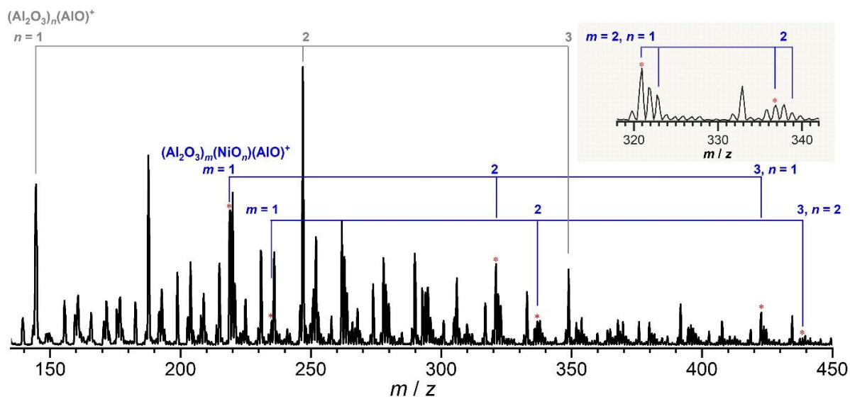
Figure 1. Quadrupole mass spectrum of the cations produced by laser ablation of an Al/Ni rod in the presence of 1% \text{O}_2 seeded in He. The dominant mass progressions are labeled.
