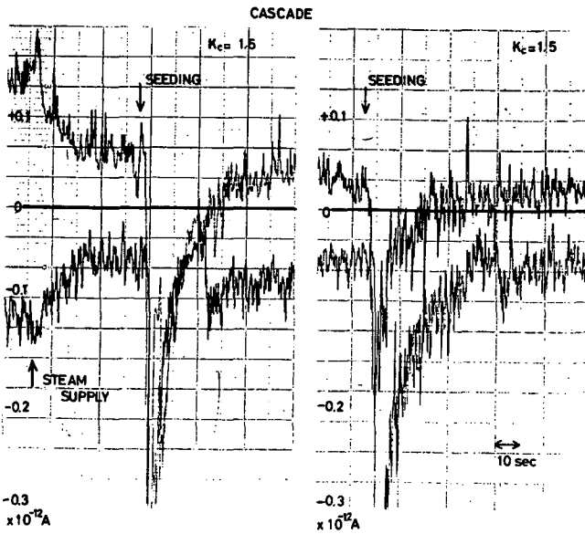
Fig. 4 Records of each polarity of ion current by the cascade method and K_c is the critical mobility in cm^2/(sec \cdot V) .
