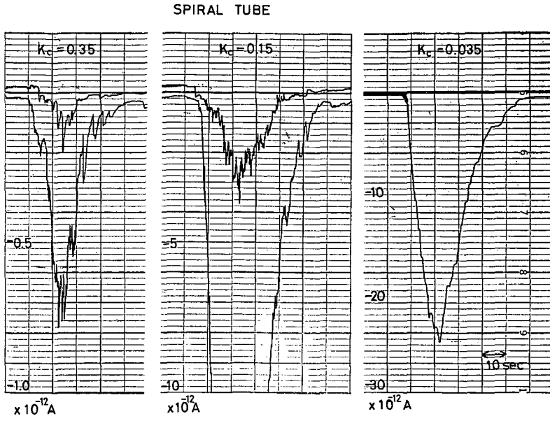
Fig. 3 Records of each polarity of ion current by spiral tube method and K_c is the critical mobility in cm^2/(sec \cdot V) .
