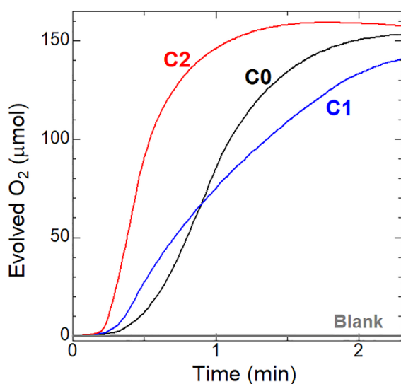
Fig. 5. Chemical OER plots of the complexes C0 (black), C1 (blue), and C2 (red) in pH = 1.0 \text{HClO}_4 aq./TFE/acetonitrile (v/v/v = 3/2/1), [CAN] = 120 mM, and [Cat.] = 100 \mu\text{M} . Gray line shows the result in the absence of a WOC.
