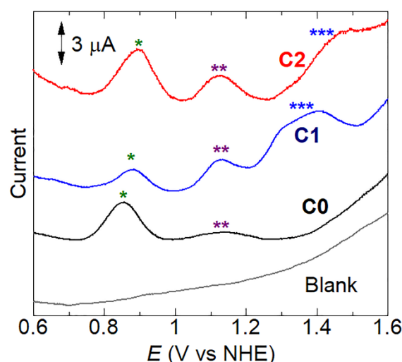
Fig. 3. DPV curves of the complexes C0 (black), C1 (blue), and C2 (red) in pH = 1.0 HClO 4 aq./TFE/acetonitrile (v/v/v = 3/2/1) containing 0.1 M NaClO 4 ; scan rate = 10 mVs -1 . Single (*), double (**), and triple asterisks (***) denote a redox couple of Ru III/II , Ru IV/III , and a cascade of Ru V/IV and (cbz ox /cbz), respectively.
