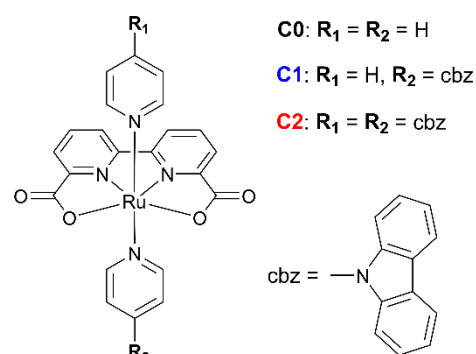
Fig. 1. Molecular structure of the complexes C0 , C1 , and C2 .
