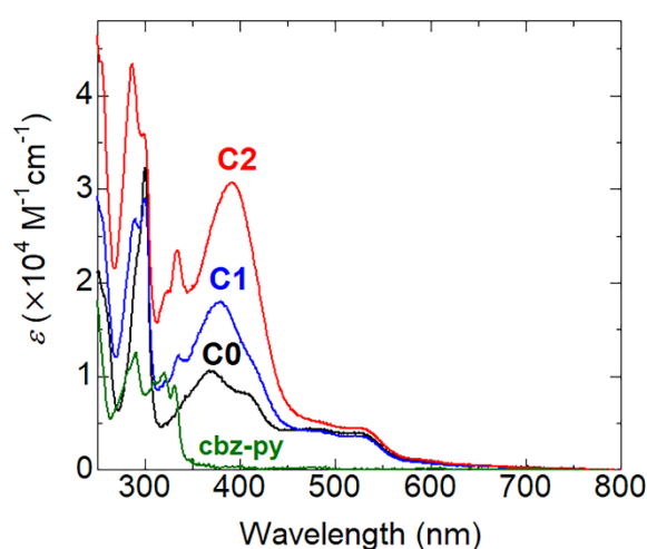
Fig. 2. UV-vis absorption spectra of the C0 (black), C1 (blue), C2 (red) complexes and cbz-py (green) ligand (10 \mu M, dichloromethane/TFE, v/v = 9/1).
