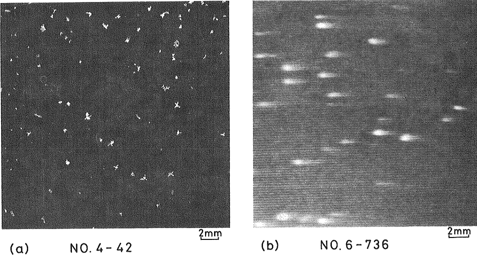
Fig. 7 A comparison of snow crystals of a combination of bullets and columns replicated on a glass slide (a) and recorded by the SCMS (b).
