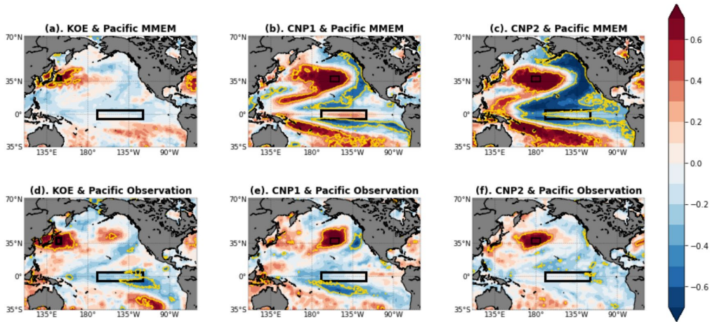
Fig. 8. Same as Fig 7, but for July.
