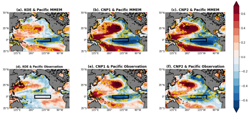
Fig. 7. (a-c) Correlation maps between area-averaged SSTA of a specific region (KOE, the CNP1, and the CNP2) and the SSTA grid point for MMEM in January. (d-f) Correlation maps with SSTA grid point for the observation, otherwise following (a-c). The black rectangles mark the areas of interest and the Niño 3.4 region. The colors indicate correlation values, and the yellow contours are significant correlations at the 95% confidence level.
