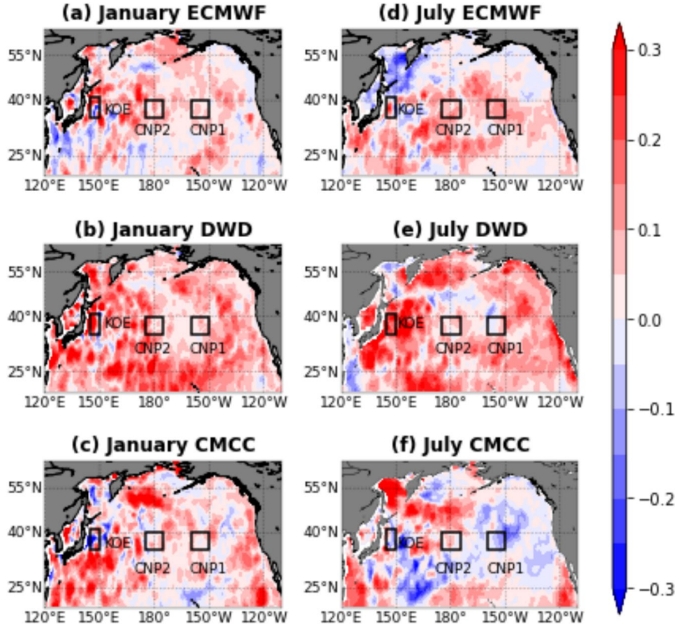
Fig. 6. The difference between MMEM prediction skill and RMEM prediction skill. The prediction skills are the point wise correlations between ensemble mean (MMEM or RMEM) and observation at each grid point. Black rectangles indicate regions of interest.
