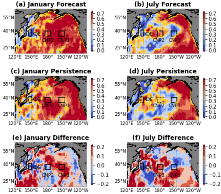
Fig. 1. (a)-(b) Prediction skill of NP based on the point-wise correlation between MMEM and observation in January and July. (c)-(d) Persistence of NP based on the point-wise correlation between observed SSTA in November (May) and January (July). (e)-(f) Difference between prediction and persistence skill. Black rectangles indicate regions of interest, i.e., the KOE, the CNP1, and the CNP2. Colors show point-wise correlation values, with yellow contours showing areas where correlations were significant at the 95% confidence level.
