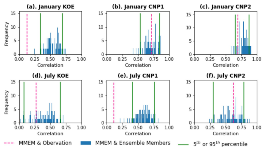
Fig. 2. Histograms of correlation distribution between the area-averaged MMEM and ensemble members (blue bars), the correlation between the MMEM and observation (vertical pink dashed line), and 5 th or 95 th percentile of correlation distribution between the MMEM and ensemble members (green lines) in January (a-c) and July (d-f) for the KOE, the CNP1, and the CNP2. The distance of the 5 th and 95 th percentile describes the ensemble spread.
