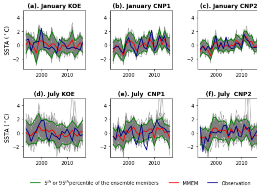
Fig. 3. Area-averaged SST anomaly (SSTA) time series of the MMEM (red), 5 th and 95 th percentile ensemble members (green), ensemble members (gray) and observation (blue) for January and July in the KOE, the CNP1, and the CNP2.
