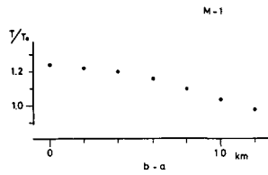
Fig. 7 Relation between the seiche period and the position of a peninsula (I). Both the length and the width of the peninsula are 3 km (in the model M-1).
