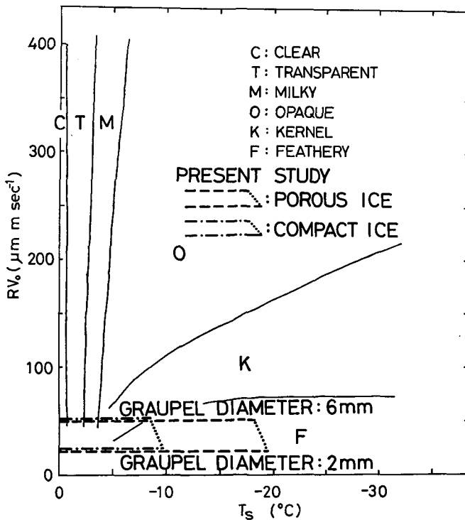
Fig. 8 The dependence of the appearance regarding graupel particles on the parameter RV_0 and the surface temperature superimposed on the diagram regarding accreted ice by Macklin (1962).
