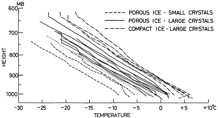
Fig. 7 Relation between characteristics of internal structure of graupel particles and vertical distributions of temperature below cloud tops.
