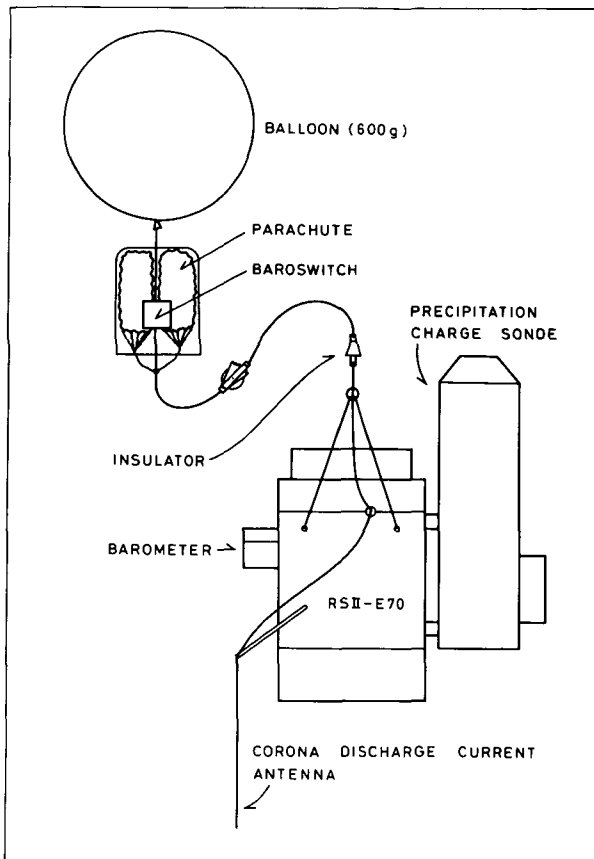
Fig. 4 Appearance of whole sonde system, not in scale.
