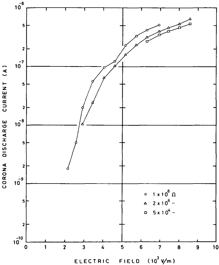
Fig. 6 Calibration curves of corona discharge current against applied electric field, for three kinds of values of resistance of input shunt.
