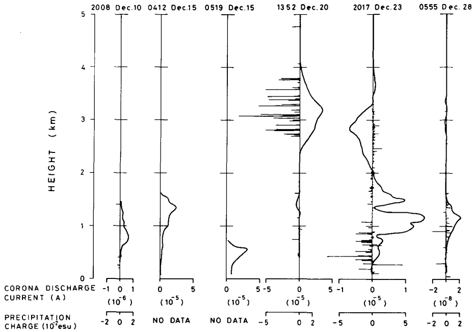
Fig. 8 Vertical distributions of electric potential gradient (solid curves) and electric charge on precipitation particles (horizontal bars).
