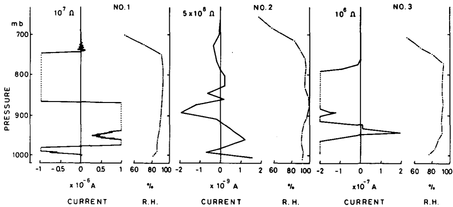
Fig. 1 Results of the preliminary test flights, which measured corona discharge current using a fixed value of resistance of input shunt.
