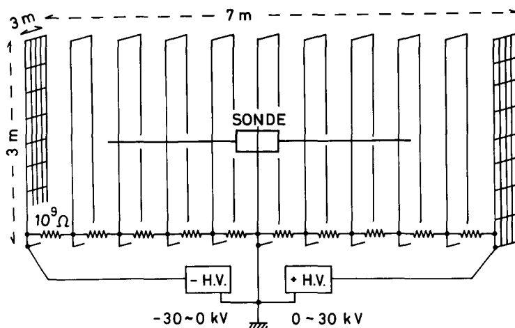
Fig. 5 Side view of the artificial electric field cage used for calibration.
