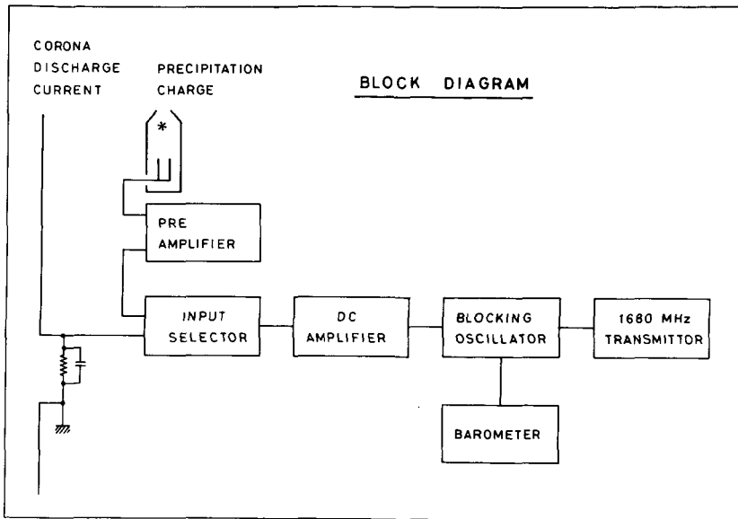
Fig. 2 Block diagram of the measuring system of specially designed sonde.
