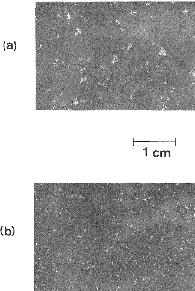
Photo.1 Typical examples of (a) "snowflake" observed 4 Jan. 1980 and (b) "no-snowflake" observed 11 Dec. 1979.
