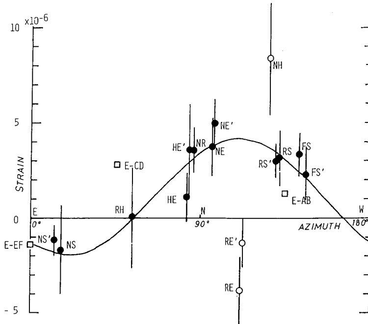
Fig. 7 Plot of the accumulated strain during the period from 1972 to 1980 versus the azimuth of base-line. Error bars represent one standard deviation on either side of the plotted point. The solid curve is the least squares solution for homogeneous plane strain excluding open circles. The results obtained by the extensometers are also shown by open square marks.
