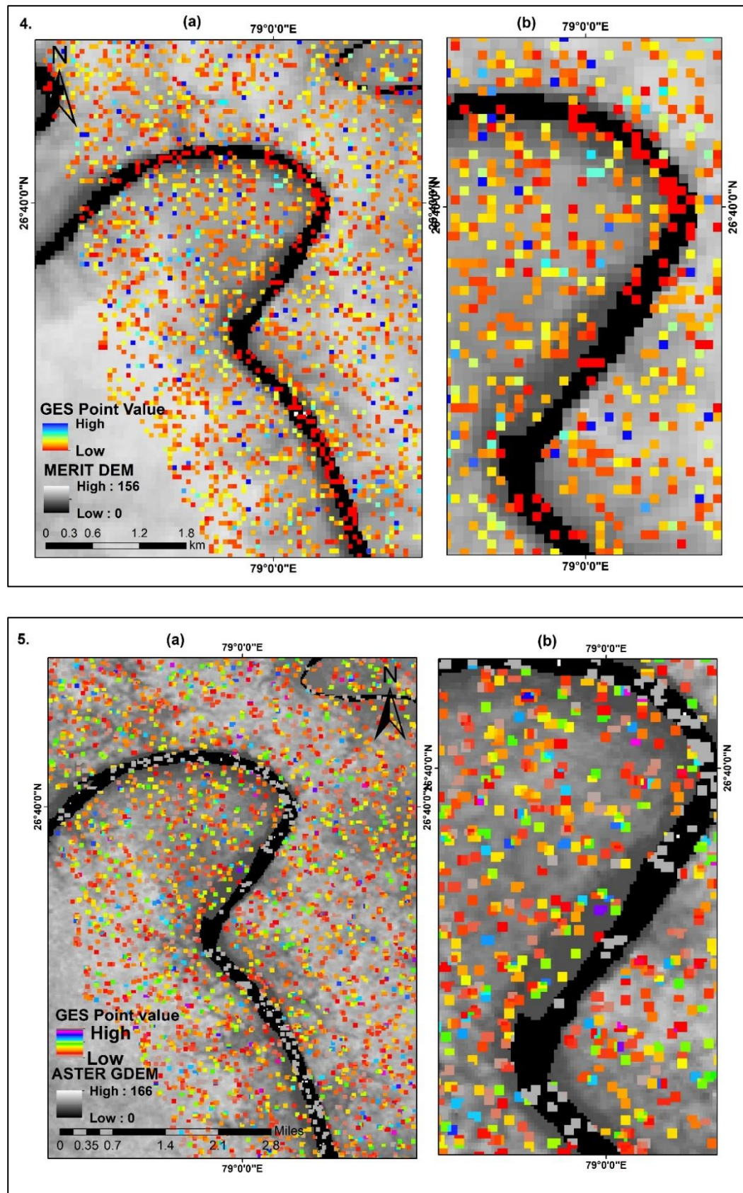
Figure 5-10: (1-5). Gully erosion Susceptibility map was deducted by using five DEM for the study area, showing in form of erosion-point value difference. (a) Erosion susceptibility location (b) Zoom extent of location.
