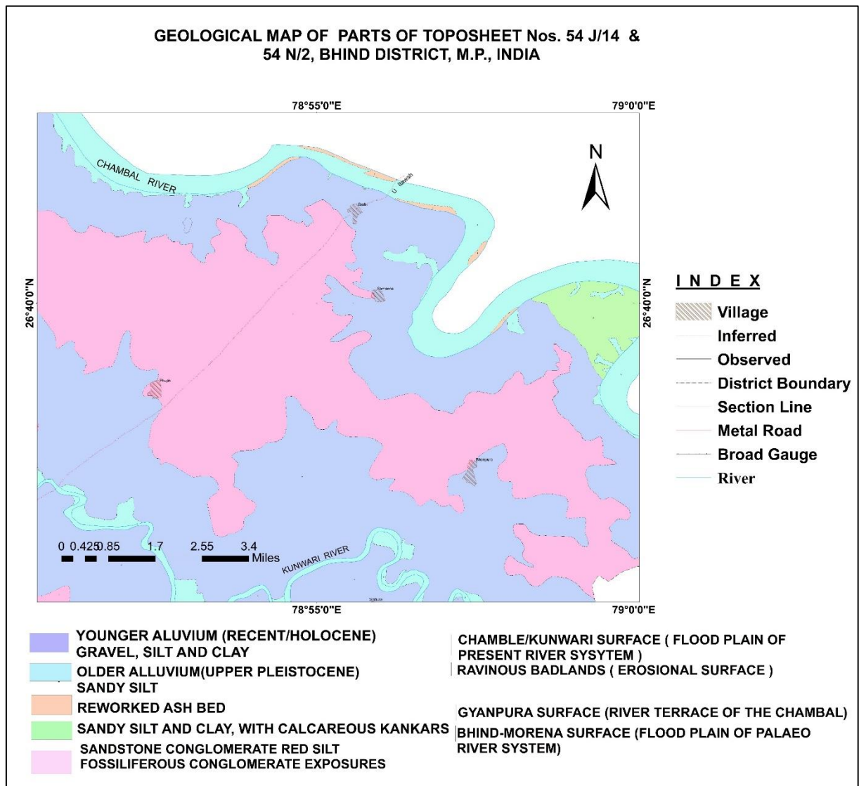
Figure 2-3: Geological Map of Chambal ravine in Bhind
