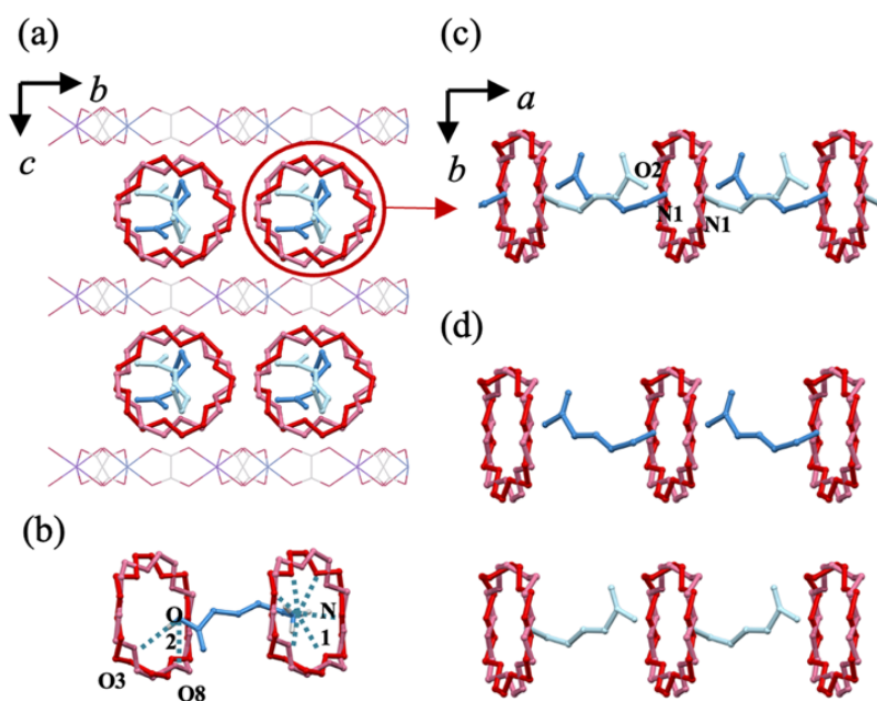
Figure 3-3. (a) Crystal structure of 5 viewed along the a -axis. (b) Hydrogen bond structure between CBA + and [18]crown-6. (c) Supramolecular column of (CBA + )([18]crown-6), viewed along the c -axis. The CBA + shows static disorder with each occupancy of 0.5 indicated by blue and light blue. The [18]crown-6 showed dynamic disorder due to Merry-go-round motion. The occupancy ratio of two molecules indicated by red and pink is 1:1. (d) Head-to-tail supramolecular cationic assembly composed of each static disorder of CBA + .
