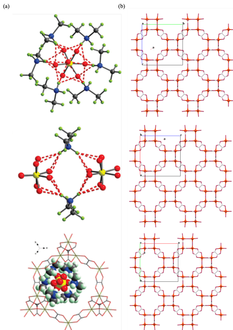
Figure 1-17. (a) D_3 symmetric supramolecular \{(\text{Me}_2\text{NH}_2)_3(\text{SO}_4)\}^+ (b) Projection of [(\text{Fe}_2(\text{oxalate})_3)]^- , viewed along a , b , and c -axis.
