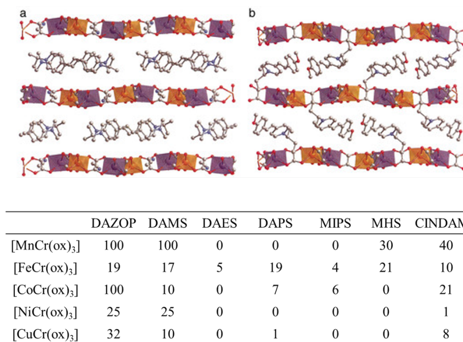
Figure 1-4. Anionic-cationic layered structure of optical active hybrid crystals (up). The SHG signals relative to Urea (below). 9
