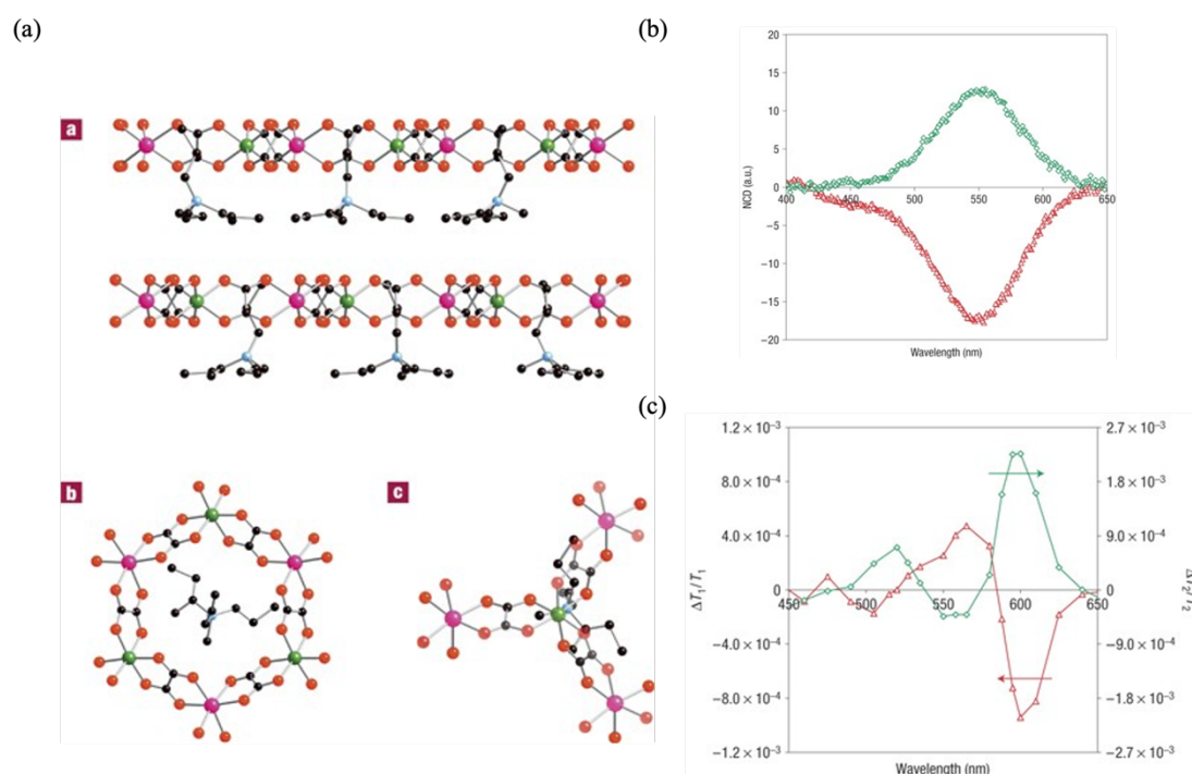
Figure 1-5. (a) Crystal structure of [\text{N}(\text{CH}_3)(n\text{-C}_3\text{H}_7)_2((S)\text{-}s\text{-C}_4\text{H}_9)][(\Delta)\text{-Mn}(\Delta)\text{-Cr}(\text{ox})_3] . (b) NCD signals of two chiral hybrid crystals. (c) Magneto-chiral dichroism measured in ferromagnetic ordering at 4 K. 10
