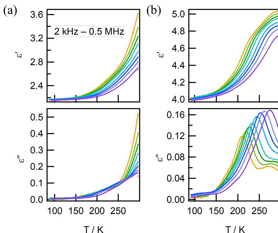
Figure 3- 4. Temperature- and frequency-dependent dielectric constants were measured on pellet samples of 5 •CH 3 OH (a) and 5 (b).
