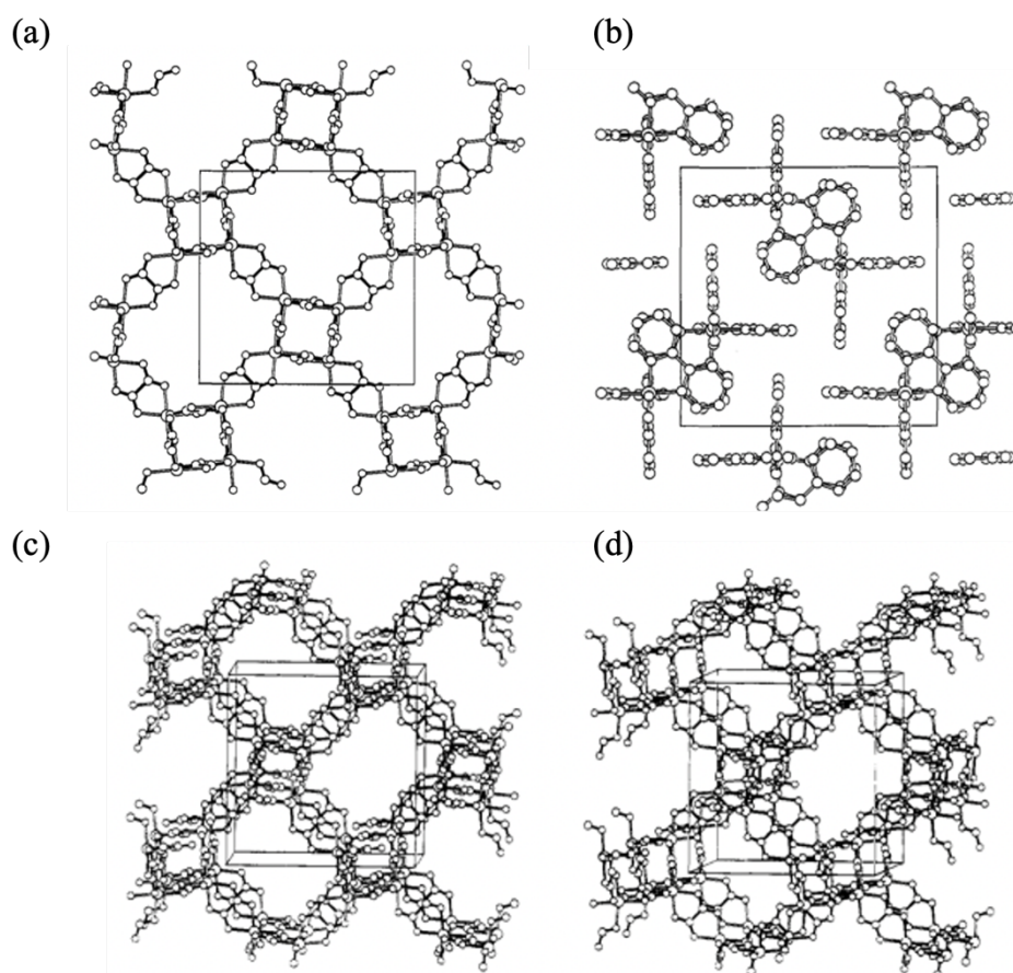
Figure 1-16. Projection of gyroid structure of [(\text{FeII})_2(\text{oxalate})_3]^- (a) (c) (d), and chiral cation [\text{Fe(II)(bpy)}_3]^+ (b).
