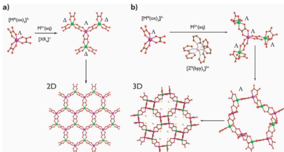
Figure 1-2. Diagram illustrating the formation of 2D heterochiral (a) and 3D homochiral (b) oxalate-based architectures depending on the nature of the templating cation. 7
