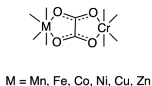
Figure 1-1. A bis-bidentate chelate form of [\text{MCr}(\text{oxalate})_3]^- (left). Schematic structure of a two-dimensional structure of [\text{MCr}(\text{oxalate})_3]^- in [\text{XR}_4][M^{II}\text{Cr}(\text{oxalate})_3] complexes. 1
