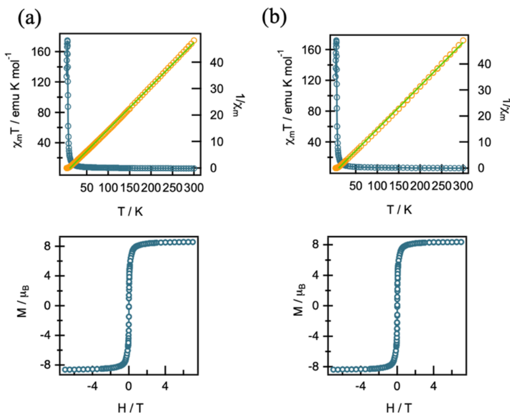
Figure 3-7. Temperature dependence of \chi_m (up) and magnetization at 1.8 K (below) for 5 •CH 3 OH(a), and 5 (b).
