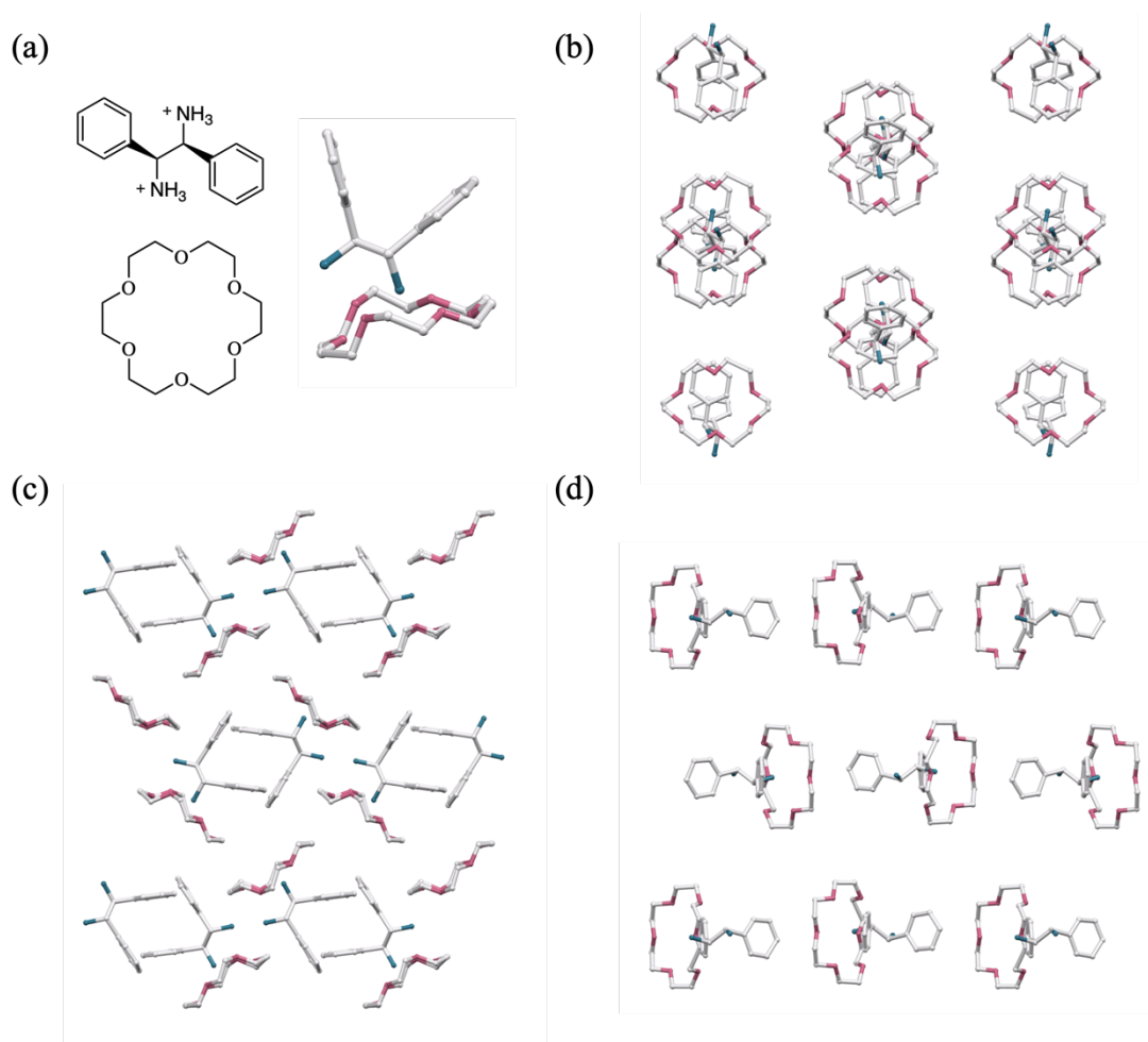
Figure 4-5. Supramolecular assembling in crystal 7.
