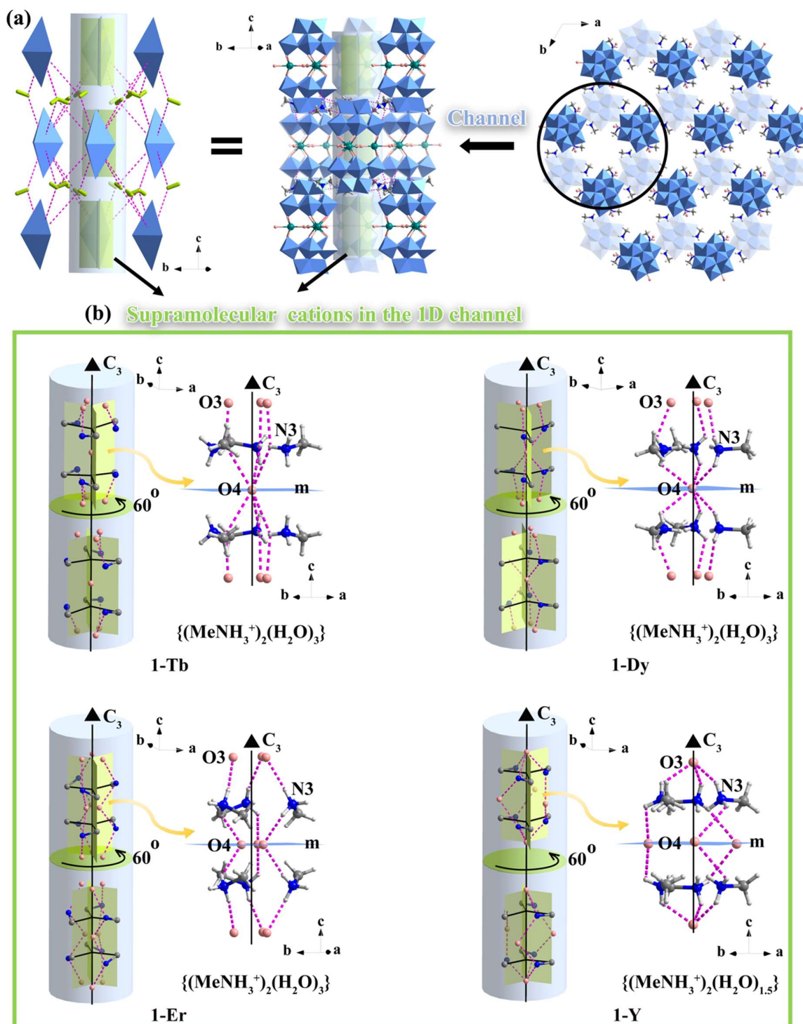
Figure 3-6. (a) Threefold symmetric one-dimensional (1D) cylindrical channels in crystal 1 . (b) The structure of hydrogen bonding supramolecular units ( \{(MeNH_3^+)_2(H_2O)_x\} ) constructed by MA^+ ( N3 ) cations and water molecules ( O3 and O4 ) accommodated in the channel of crystal 1 . Hydrogen bonding is shown in magenta dotted line.
