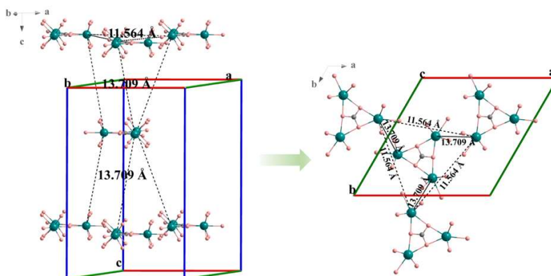
Figure 3-8. The distance between \text{Tb}^{3+} ions of sandwich POM anions of crystal 1-Tb .
