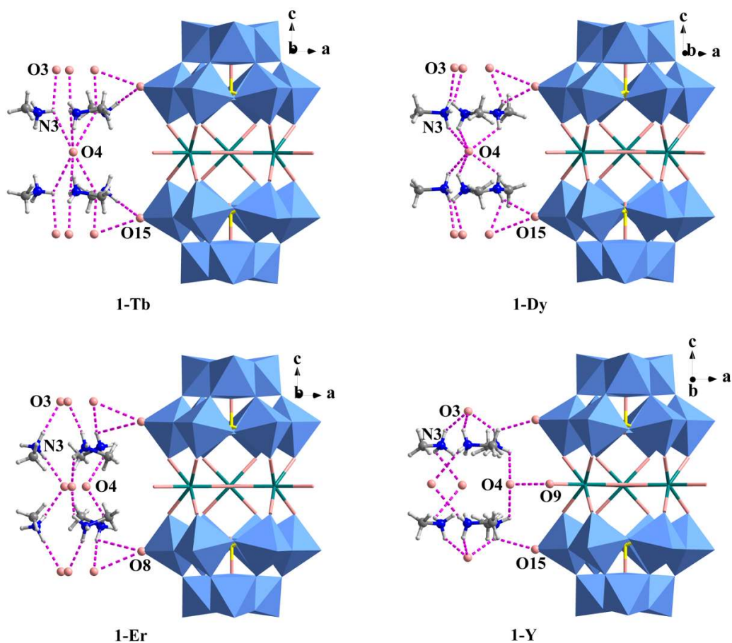
Figure 3-7. The hydrogen bonding interaction between \{(\text{MeNH}_3^+)_2(\text{H}_2\text{O})_x\} units existing in channel and surrounding sandwich POM anions in crystal 1 . Hydrogen bonding is shown in magenta dotted line.
