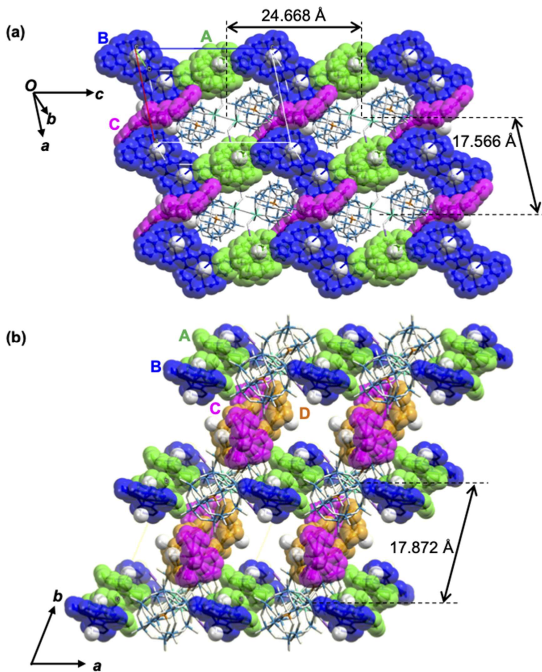
Figure 4-7. Packing structure of crystal 6-Dy viewed along the (a) b and (b) c axes. The central F - distances between adjacent Dy 2 POMs are given in the figure.
