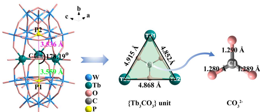
Figure 3-10. The structure of sandwich POM anion in crystal 2 . The distorted triangle structure constructed by \{\text{TbCO}_3\} unit (Middle). The structure of \text{CO}_3^{2-} in \{\text{TbCO}_3\} unit (right). The distance between P1 and C1 and the distance between P2 and C1 are shown in light green and magenta, respectively.
