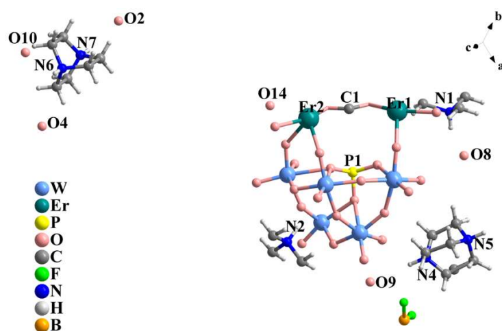
Figure 3-20. The asymmetric unit of crystal 5-Er .
