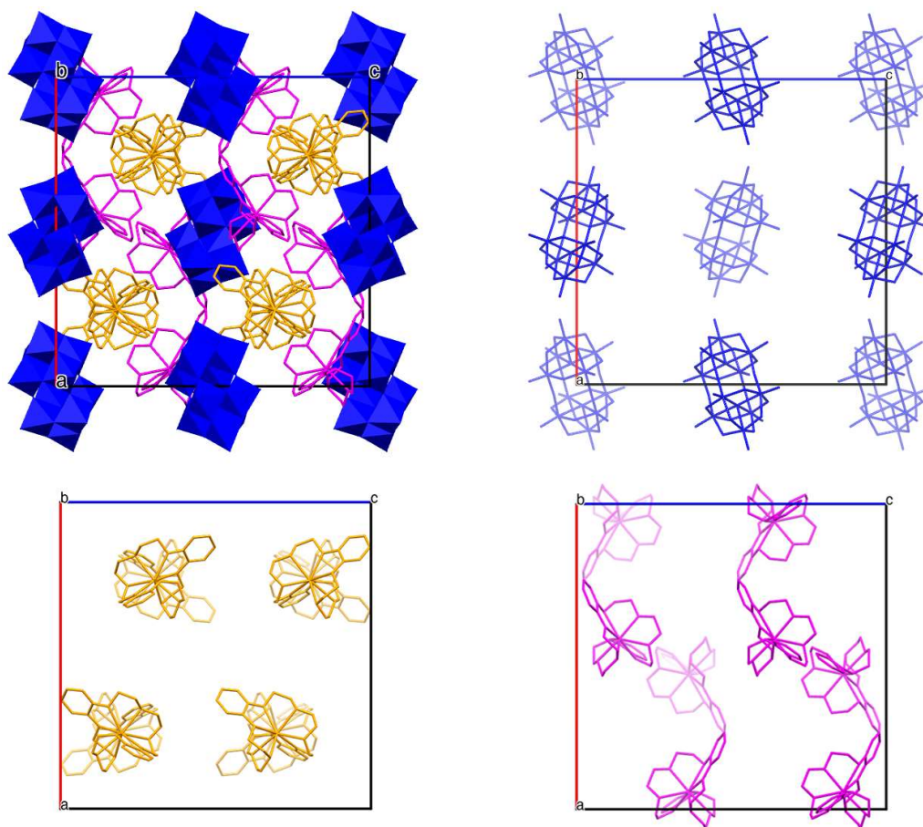
Figure 9. (a) The packing structure of crystal 8 . (b) The packing structure of [\text{W}_{10}\text{O}_{32}]^{4-} anions in the crystal. (c) The packing structure of [(\text{Na}^+)(\text{DB}[24]\text{crown-8})] supramolecular cations of A in the crystal. (d) The packing structure of [(\text{Na}^+)(\text{DB}[24]\text{crown-8})] supramolecular cations of B in the crystal. [(\text{Na}^+)(\text{DB}[24]\text{crown-8})] supramolecular cations are shown in stick models. [\text{W}_{10}\text{O}_{32}]^{4-} anions in (a) and (b) are shown in blue polyhedral and blue stick model, respectively.
