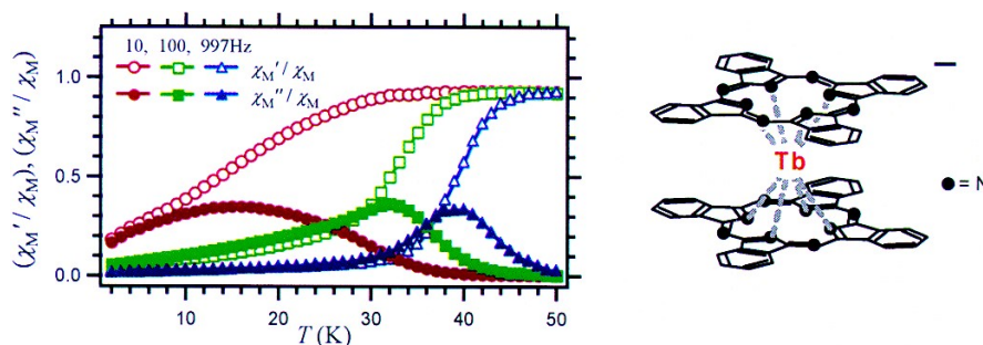
Figure 1-10. The dynamic magnetic properties and molecular structure of double-decker phthalocyanine complexes [\text{TbPc}_2]^- \text{TBA}^+ . 102
