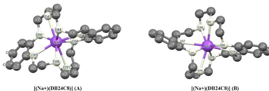
Figure 7. Crystallographically independent structure of (Na + )(DB[24]crown-8) units ( A and B ) in crystal 8 at 94 K. Hydrogen atoms are omitted for clarity. Gray, white and purple atoms correspond to carbon, oxygen and sodium, respectively. Hydrogen atoms are omitted for clarity.
