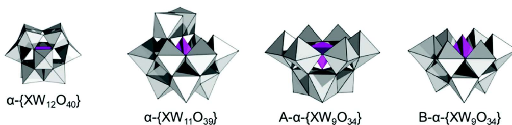
Figure 1-6. Polyhedral representation of the saturated \alpha -Keggin POMs and the related “unsaturated” POMs (lacunary POMs). 77
