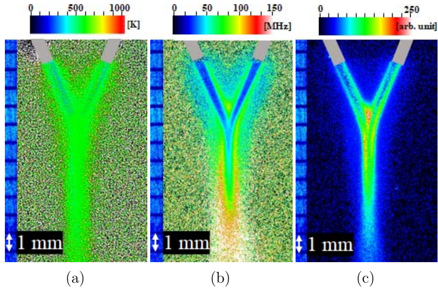
Figure 8. Two dimensional maps of (a) rotational temperature of \text{OH}(X^2\Pi(v'' = 0)) , (b) destruction frequency of laser-excited \text{OH}(A^2\Sigma^+) , and (c) OH radical density. The discharge conditions were the same as those in Fig. 5.
