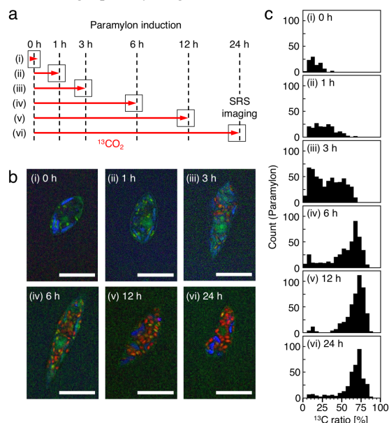
Figure 4. Time-resolved SRS imaging of paramylon granule-incorporated ^{13}\text{C} with a ^{13}\text{C} source. (a) Timeline of the incubation of the E. gracilis cells with ^{13}\text{C} incubation. (b) SRS images of the E. gracilis cells. The ^{13}\text{C} and ^{12}\text{C} constituents as well as the chloroplasts were color-coded in red, green, and blue in the RGB color model, respectively, employing the spectra in Figure 2a. Scale bars: 20 \mu\text{m} . (c) Histograms of the ^{13}\text{C} ratios of the paramylon granules. The ^{13}\text{C}
