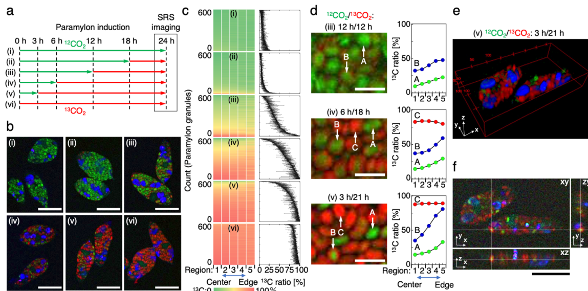
Figure 5. SRS imaging of the E. gracilis cells and their paramylon granules that were incubated via atmospheric switching from the ^{12}\text{C} to the ^{13}\text{C} source. (a) Incubation timeline of the E. gracilis cells with incubation switching from the ^{12}\text{C} to ^{13}\text{C} source at different periods. (b) Representative SRS images of the E. gracilis cells that were incubated under the conditions in (a). All the measured SRS images are shown in Figure S4. Scale bars: 20\ \mu\text{m} . (c) Heatmaps (left) and average values with standard deviations (right) of the ^{13}\text{C} ratios in the five segmented regions (from the center to the periphery) of the individual paramylon granules ( n = 600 ). The ^{13}\text{C} ratios were calculated by analyzing the SRS images ( n = 9 , including the images in (b)). (d) Left: Magnified SRS images of the extracted paramylon granules that were incubated under the conditions in (iii), (iv), and (v) of (a). Representative granules ( ^{12}\text{C} -rich, A; ^{13}\text{C} -localized, B; ^{13}\text{C} -rich, C) are indicated by arrows. Scale bars: 5\ \mu\text{m} . Right: Plots of the ^{13}\text{C} ratios of the corresponding granules against the five segmented regions. (e) Three-dimensional SRS imaging of the E. gracilis cells that were incubated under the condition in (v) of (a). (f) Cross-sectional analysis of the E. gracilis cells in image (e). Scale bars: 20\ \mu\text{m} . The ^{13}\text{C} and ^{12}\text{C} constituents, as well as the chloroplast in all the SRS images, correspond to the red, green, and blue color codes in the RGB color model, respectively, employing the spectra in Figure 2a or Figure S9a.
