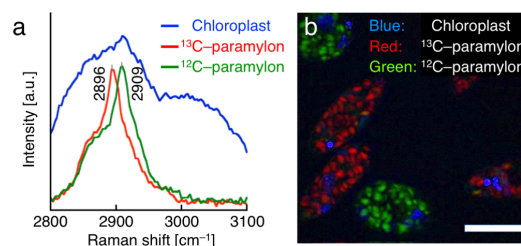
Figure 2. SRS imaging of the mixed E. gracilis cells accumulating ^{13}\text{C} - or ^{12}\text{C} -paramylon granules. (a) Raman spectra of the ^{13}\text{C} - and ^{12}\text{C} -paramylon granules as well as the chloroplasts in the CH stretching region ( 2800\text{--}3100\text{ cm}^{-1} ). Red: ^{13}\text{C} -paramylon granules, green: ^{12}\text{C} -paramylon granules, blue: chloroplasts. (b) An SRS image of the mixed cells. The three constituents ( ^{13}\text{C} - and ^{12}\text{C} -paramylon granules, as well as the chloroplasts) are color-coded in red, green, and blue in the RGB color model, respectively. Scale bar: 20\text{ }\mu\text{m} .
