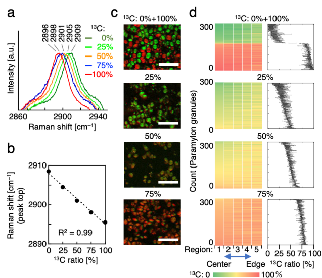
Figure 3. SRS microscopy and statistical analyses of the extracted paramylon granules that were incubated with the ^{13}\text{C} and ^{12}\text{C} sources in different molar ratios. (a) Enlarged view of the Raman spectra peaks in the CH stretching region of the paramylon granules that were incubated in different ratios of the ^{13}\text{C} source. (b) Raman shifts of the peaks against the ratios of the ^{13}\text{C} source in the culture media. (c) SRS images of the extracted paramylon granules, which were color-coded as red and green employing the spectra of the 100% ^{13}\text{C} - and 100% ^{12}\text{C} -paramylon granules, respectively, in the RGB color model. The granules were mixed in the cases of the 0% and 100% ^{13}\text{C} sources. Scale bars: 10 \mu\text{m} . (d) Heatmaps (left) and average values with standard deviations (right) of the ^{13}\text{C} ratios in the five segmented regions (from the center to the periphery) of the individual paramylon granules ( n = 300 ). The ^{13}\text{C} ratios were calculated by analyzing the SRS images ( n = 5 , including the images in (c)).
