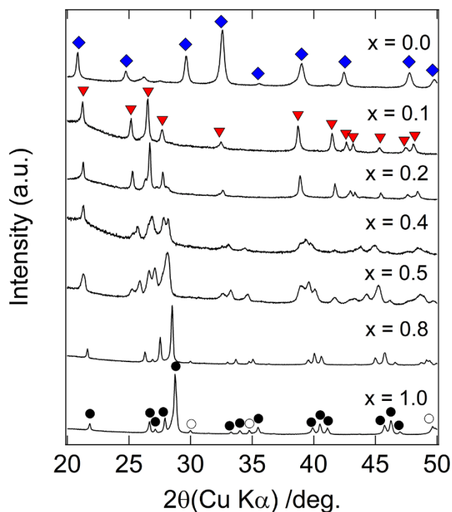
Figure 1 XRD patterns of nitrated products obtained from (\text{Ba}_{1-x}\text{Sr}_x)\text{CO}_3 precursors with x = 0\sim 1 . Diffraction lines marked with blue diamonds, red triangles, filled circles and open circles indicate tetragonal \text{BaNCN} , the novel crystalline phase, orthorhombic \text{SrNCN} and \text{SrO} , respectively.
