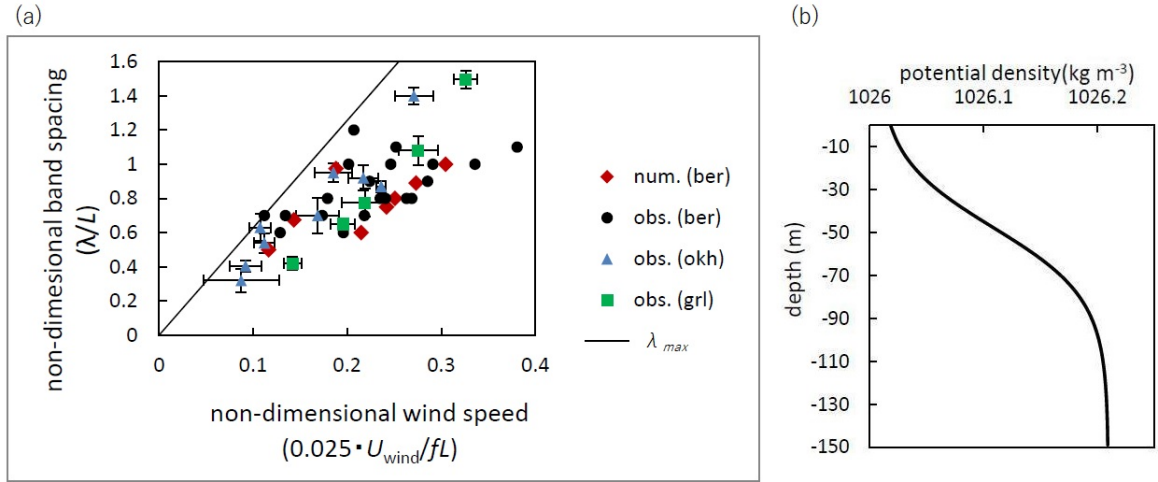
Figure 15: (a) Relationship between non-dimensional wind speed and non-dimensional band spacing. "obs.(ber)" denotes the results of the Bering Sea observations (redrawn from Muench and Charnell , 1977, Fig. 5). "obs.(okh)" denotes the results of the Okhotsk Sea observations. "obs.(grl)" denotes the results of the East Greenland Current observations. The solid line denotes \lambda_{max} = 2\pi\bar{U}_i/f . The error bar denotes the standard deviation. Note that the scale of L is 10 km, U_i is 2.5% of the 10 m wind and f is 1.12 \times 10^{-4} \text{ s}^{-1} . (b) Initial density profile of the numerical experiments in Fig. 15a, denoted by "num.(ber)", which represents a typical profile of the winter Bering Sea (e.g. Muench et al. , 1983, Fig. 5). The potential density profile is given by 0.1 \tanh\{0.03(z - 50)\} + 1026.105 , with z denoting the depth.
