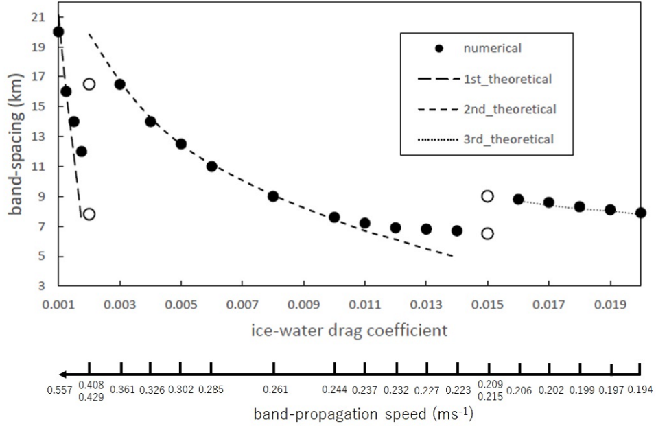
Figure 21: Relationship between ice-water drag coefficient C_{Diw} and band spacing \lambda . \bullet denotes numerical results. \circ denotes cases that give two numerical values for a single drag coefficient. Three curves in this figure denote theoretical results of 1st, 2nd, and 3rd modes, respectively, evaluated by the band propagation speed with varying C_{Diw} .
