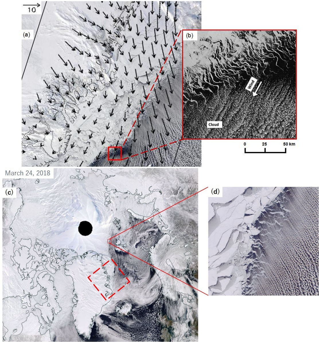
Figure 1: (a) Satellite images of ice-band patterns on March 21, 2010, from Moderate-Resolution Imaging Spectroradiometer (MODIS) images by the National Aeronautics and Space Administration (NASA) [URL: http://lance-modis.eosdis.nasa.gov/imagery/subsets/?mosaic=Arctic ]. Wind vectors ( \text{ms}^{-1} ) are derived from 10 m wind vectors of ERA-Interim (Dee, D. P. et al., 2011) (b) Enlarged view in the red box of Fig. 1a shows ice bands. (c) Satellite images of ice-band patterns in the Eurasian Basin of the Arctic Sea on March 24, 2018, from MODIS [URL: http://lance-modis.eosdis.nasa.gov/imagery ]. The domain of Fig. 1a is denoted by a red dashed box on Fig. 1c. (d) Enlarged view in the red box of Fig. 1c showing ice bands.
