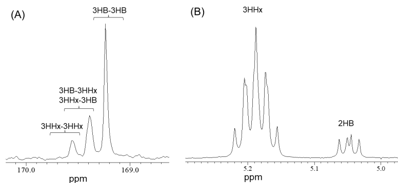
Figure 5. ^{13}\text{C} NMR of carbonyl carbons in P(3HB-co-3HHx) (A) and ^1\text{H} NMR of methine protons in binary polymer containing 3HHx and 2HB (B). The polymers in (A) and (B) were obtained by using PhaC AR F314H. Full spectra are shown in Figures S3 and S4, respectively.
