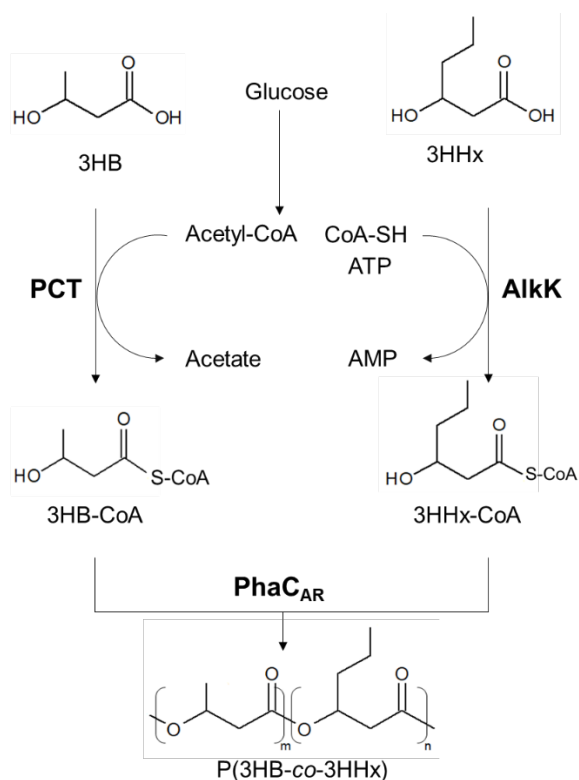
Figure 1. Metabolic pathway used in the study. The monomer precursors, 3HB and 3HHx, are supplemented into the medium. PCT and AlkK serve as monomer supplying routes for 3HB-CoA and 3HHx-CoA, respectively.
