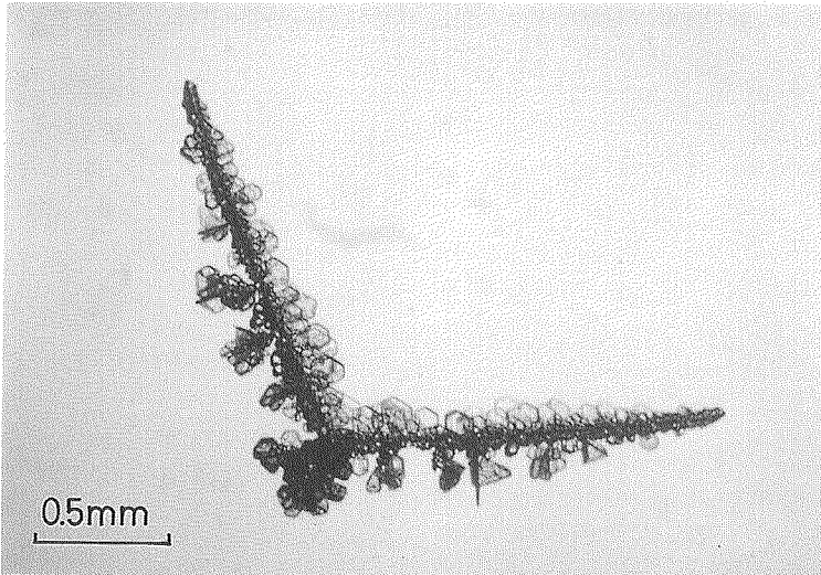
Fig. 1 A microphotograph of typical examples of the sea gull type crystals.
