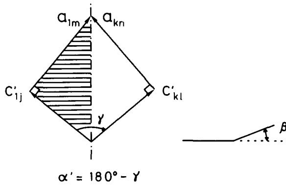
Fig. 3 Angles of \alpha' and \beta of the gohei twin type crystals (Kikuchi and Sato, 1984).
