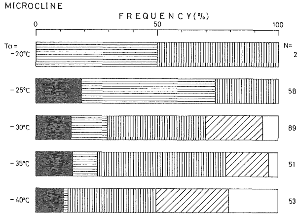
Fig. 10 Production ratio of ice crystals at each temperature on microcline.
