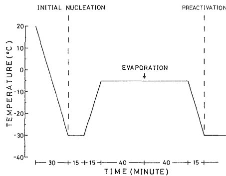
Fig. 14 Temperature history in the cold chamber at preactivation.
