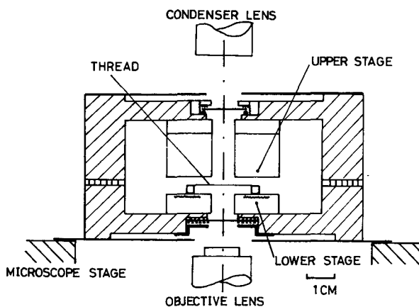
Fig. 1 Schematic diagram of the thermal diffusion type cold chamber.
