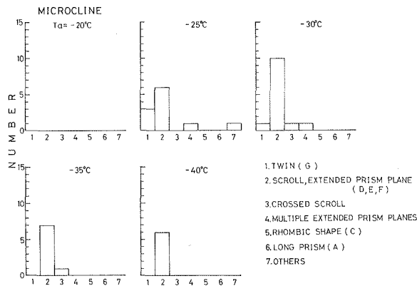
Fig. 11 Number frequency of peculiar crystals.
