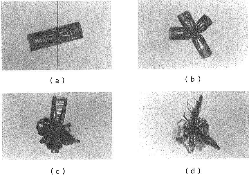
Fig.5 Examples of each type of ice crystals. (a) column, (b) combination of columns, (c) combination of columns and plates and (d) radiating assemblage of plates.
