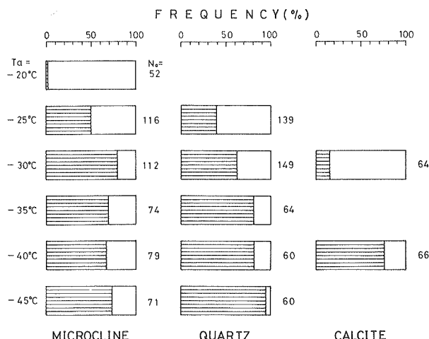
Fig. 12 Change of nucleation ratio with temperature on microcline, quartz and calcite.
