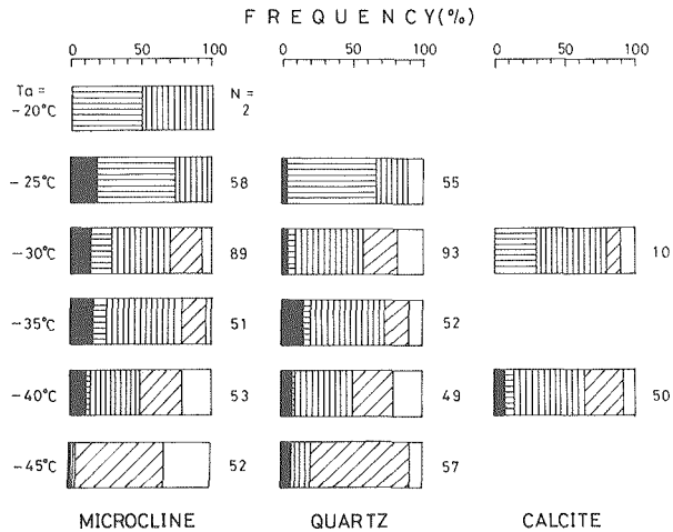
Fig. 13 Change of production ratio of various types of ice crystals with temperature.
