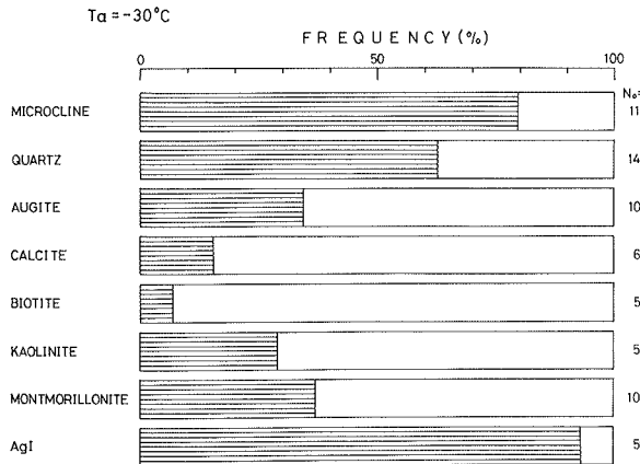
Fig. 4 Nucleation ratio on each substance of ice nuclei.
