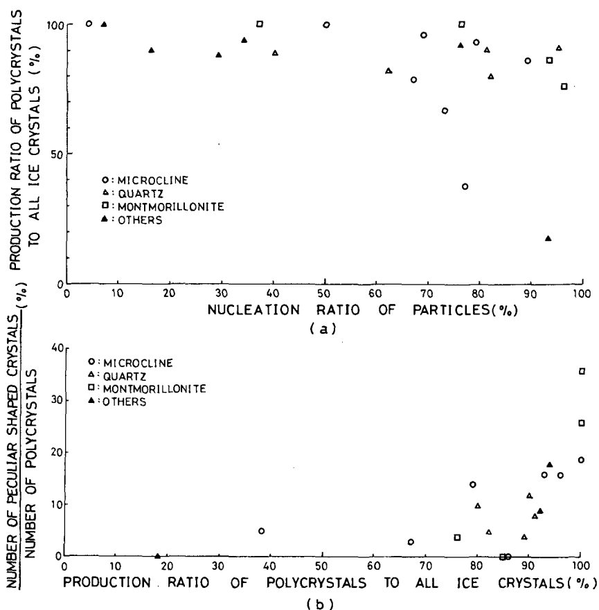
Fig. 18 (a) The relationship between nucleation ratio and production ratio of polycrystals. (b) The relationship between production ratio of polycrystals and that of peculiar shaped crystals.
