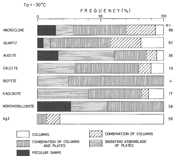
Fig.6 Production ratio of ice crystal shape at -30^\circ\text{C} .
