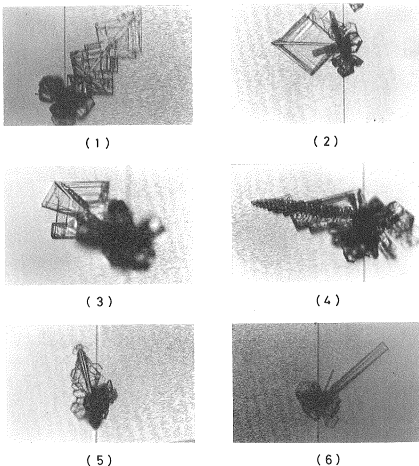
Fig. 7 Examples of peculiar shapes. (1) twin, (2) scroll and extended prism plane, (3) crossed scroll, (4) multiple extended prism planes, (5) rhombic shape and (6) long prism.
