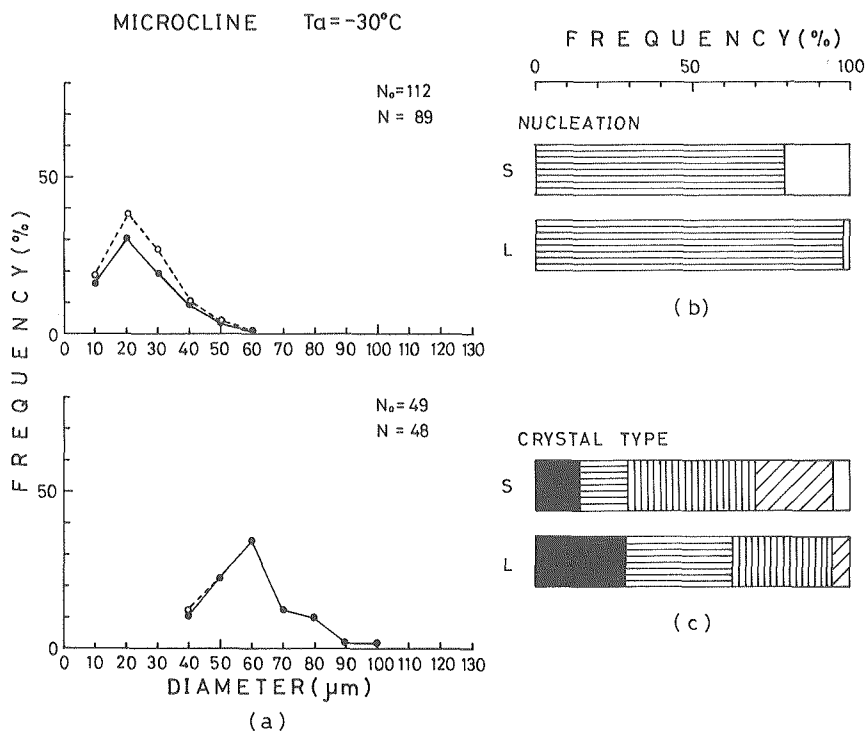
Fig. 16 Size effect of ice nuclei. (a) size distribution of smaller group and larger group of ice nuclei, (b) nucleation ratio of each group and (c) production ratio of various types of ice crystals of each group.
