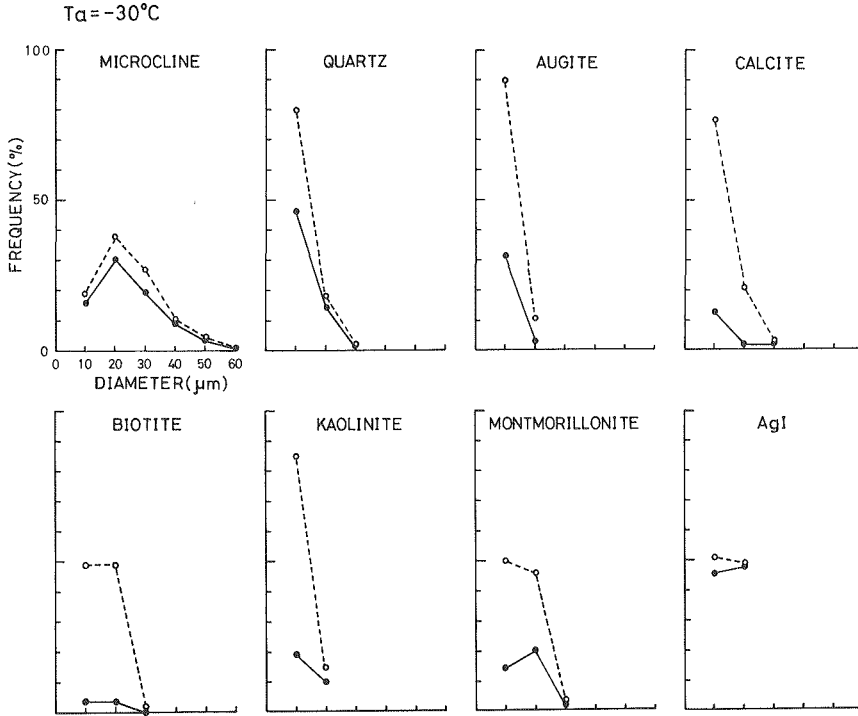
Fig. 3 Size distribution of particles of each substance.
