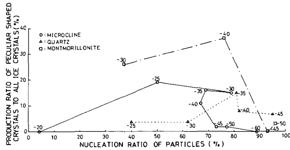
Fig. 19 The relationship between nucleation ratio and production ratio of peculiar shaped crystals.
