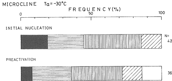
Fig. 15 Production ratio of various types of ice crystals at initial nucleation and preactivation.
