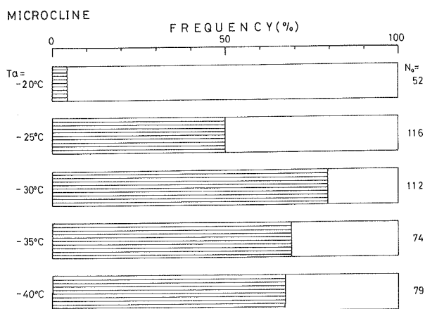
Fig. 9 Nucleation ratio at each temperature on microcline.
