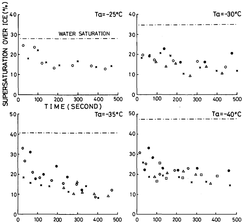
Fig.2 Supersaturation in cold chamber as a function of time when T_a was -25^\circ , -30^\circ , -35^\circ and -40^\circ\text{C} .
