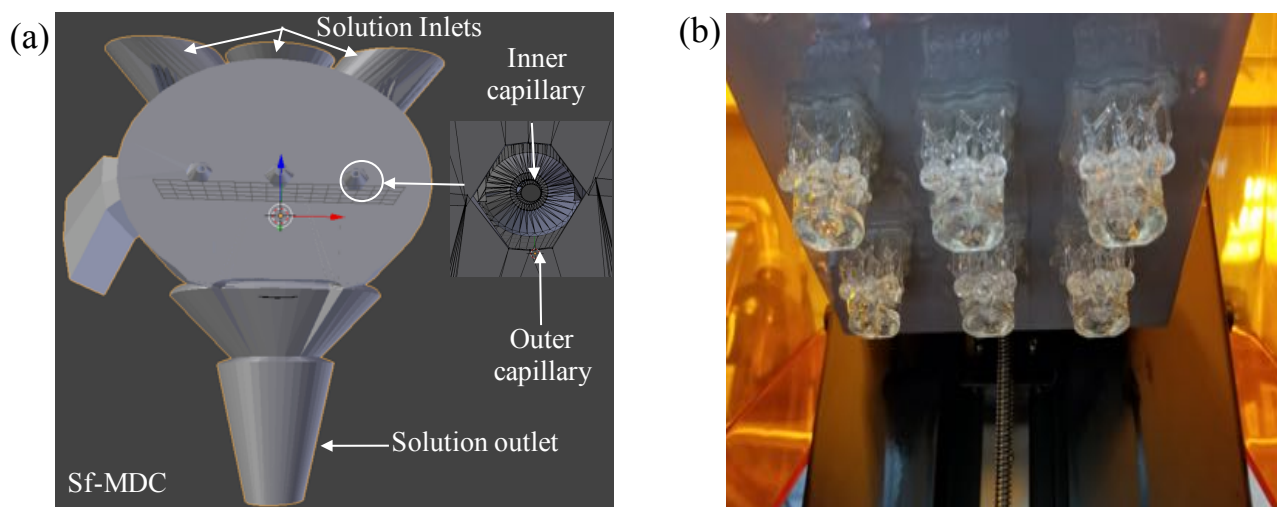
Fig.1 Top view of Sf-MDC obtained from CAD software, (a), and the image showing multiple Sf-MDC printed at once (b).
