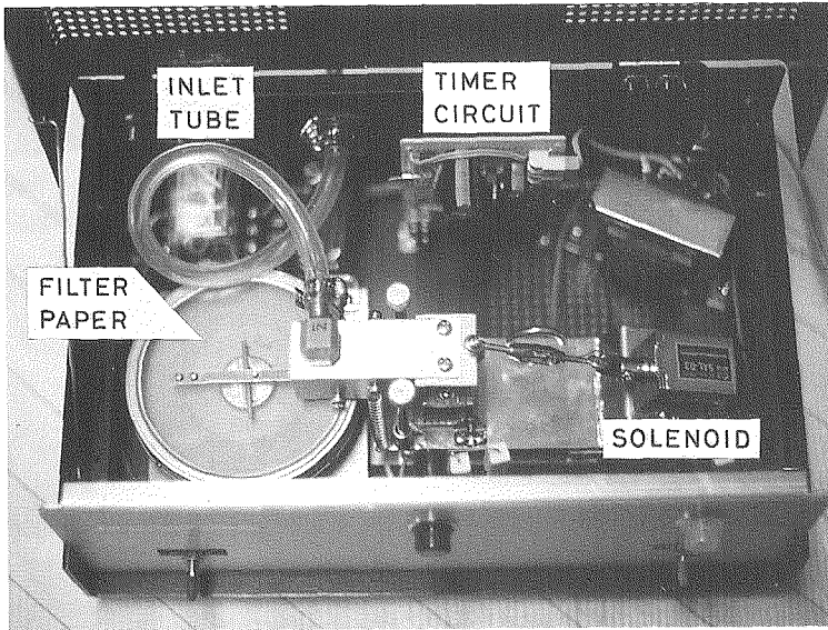
Fig. 1 A plan view of the continuous aerosol sampler.
