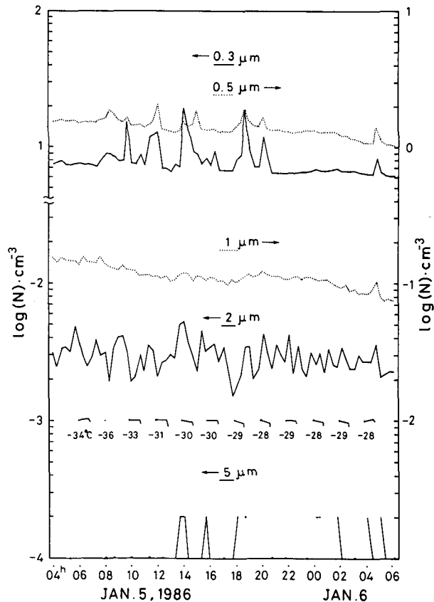
Fig. 5 An example of the time change of non-polluted day.
