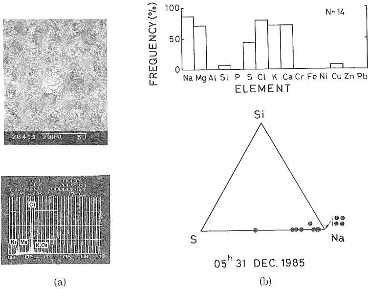
Fig. 8 (a): SEM image of a particle (upper) and chemical components included in this particle (lower). Horizontal bar indicates 5 μm. (b): Frequency of detection for each elements (upper) and triangular diagram of the typical three elements of Si, Na and S (lower).
