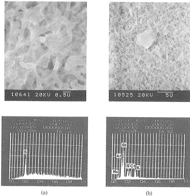
Fig. 12 Same as in Fig. 10, but for diamond dust days. (a): sulfur particle, (b): composite particle. Horizontal bar in (a) indicates 0.5 \mu\text{m} .
