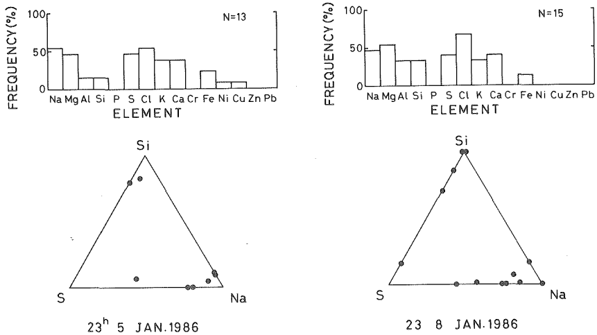
Fig. 9 Chemical components detected from the sample on easterly wind days.
