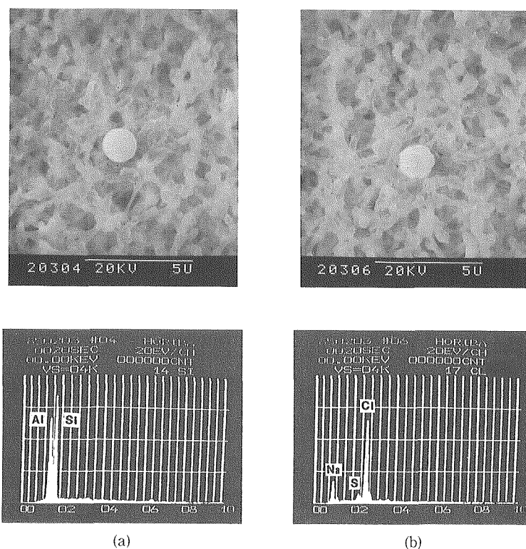
Fig. 10 Typical aerosol particles and their chemical components on easterly wind days. (a): soil particle, (b): sea salt particle.
