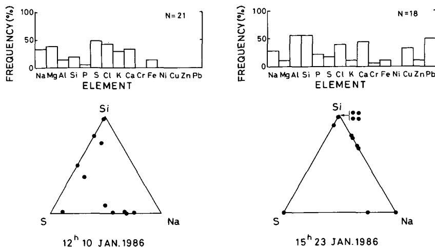
Fig. 13 Same as in Fig. 9, but for polluted days.
