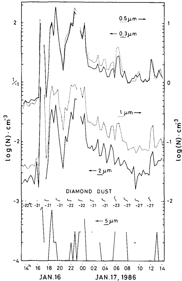
Fig. 7 An example of the time change of westerly wind day.
