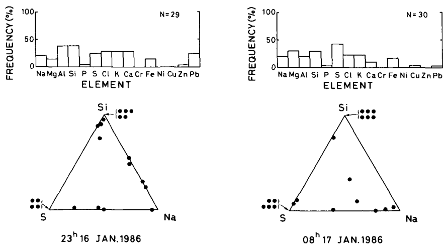
Fig. 11 Same as in Fig. 9, but for diamond dust days.
