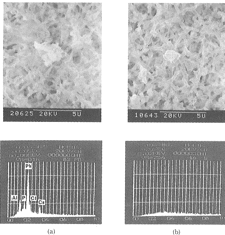
Fig. 14 Same as in Fig. 10, but for polluted days. (a): particles containing considerable lead, (b): carbon particle.
