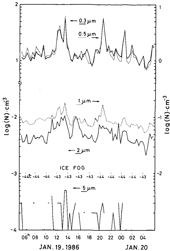
Fig. 6 An example of the time change of ice fog day.
