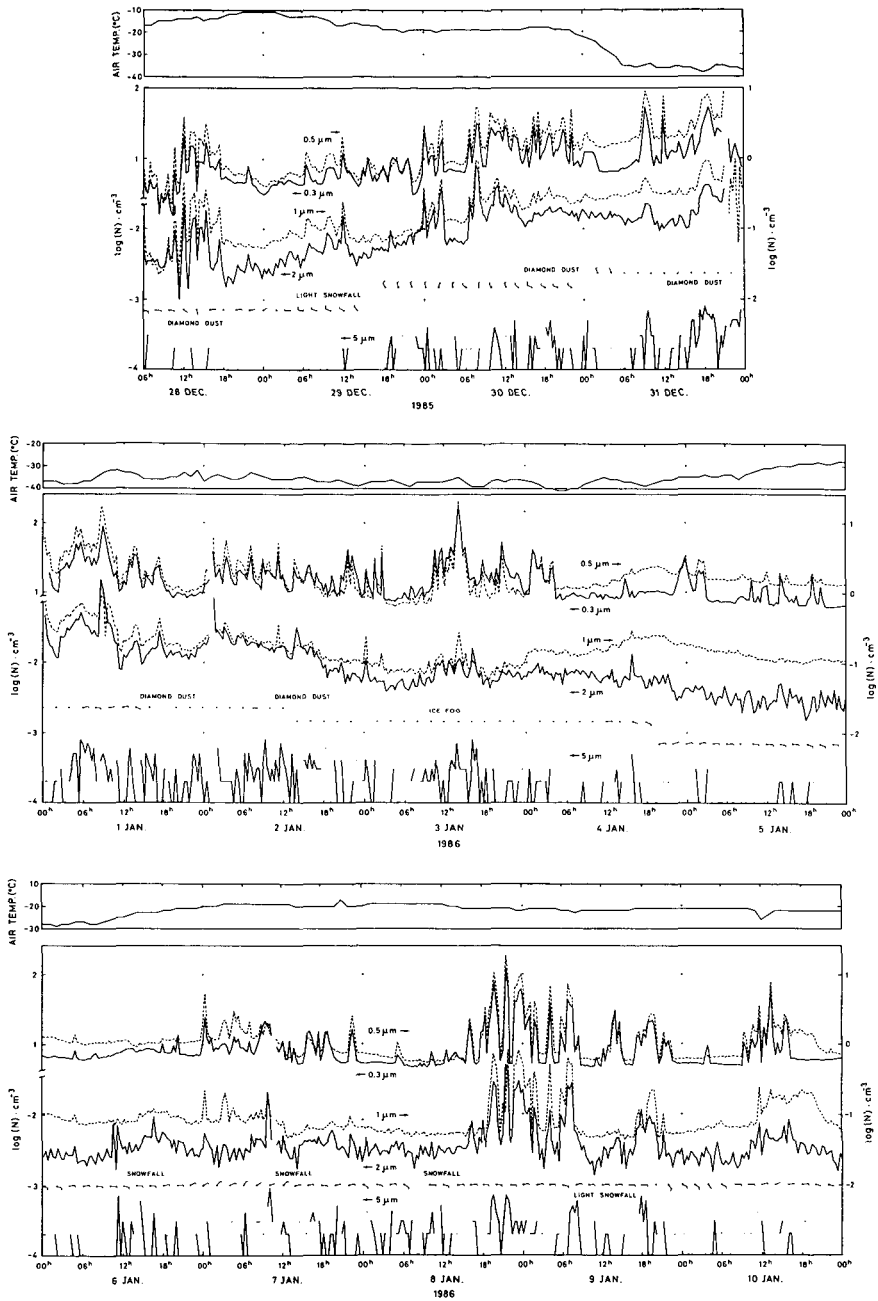
Fig. 4 Time changes of the number concentration of aerosol particles and meteorological conditions.
