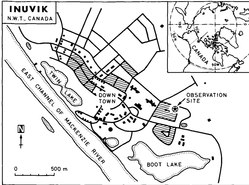
Fig. 3 Location of the observation site.
