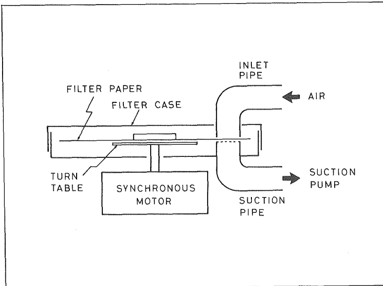
Fig. 2 The mechanical part of the continuous aerosol sampler.
