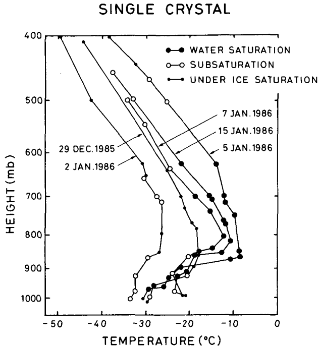
Fig. 18. Same as Fig. 17 but for single crystals were falling mostly.
