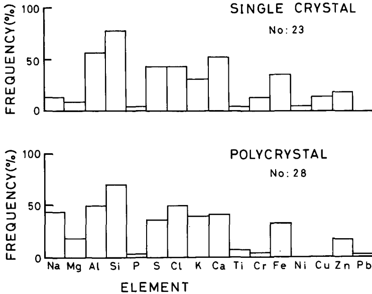
Fig. 10. Frequency distributions of the elements of single and polycrystals.
