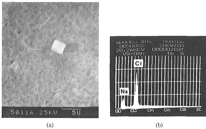
Fig. 12. Analysis of aerosol particles. (a) SEM photograph, (b) EMAX spectrum.
