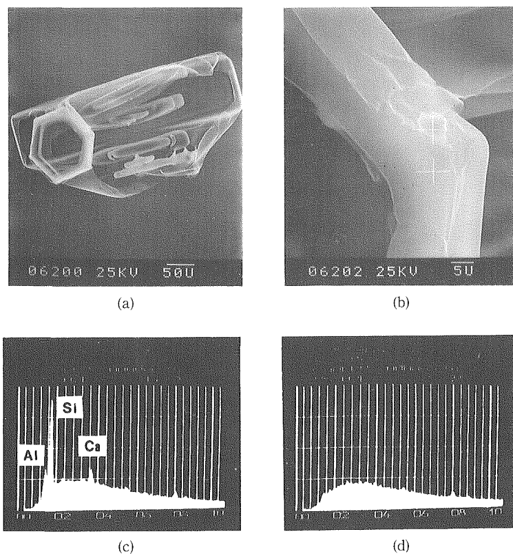
Fig. 4. Same as Fig. 3 but for column.
