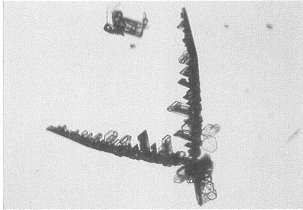
Fig. 8. Same as Fig. 6 but for the sea gull type crystal ( \times 35 ).
