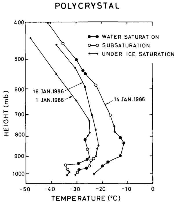
Fig. 17. Sounding curves when the polycrystalline snow crystals were falling mostly.
