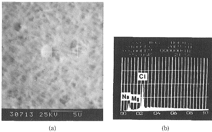
Fig. 13. Same as Fig. 12. (a) SEM photograph, (b) EMAX spectrum.
