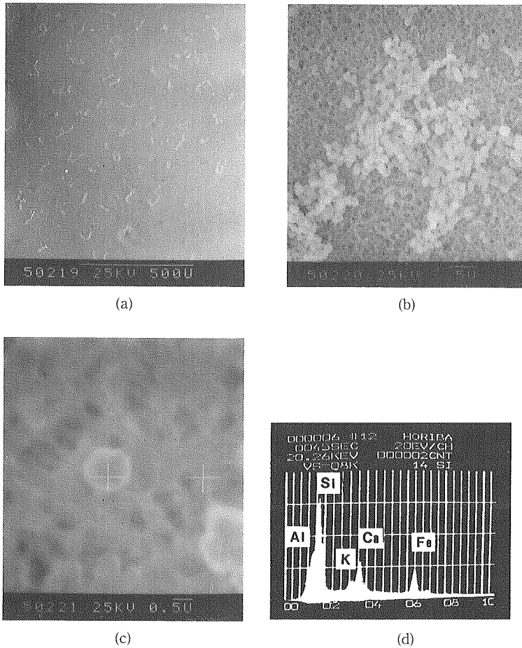
Fig. 14. Same as Fig. 12. (a), (b) and (c) SEM photographs, (d) EMAX spectrum.
