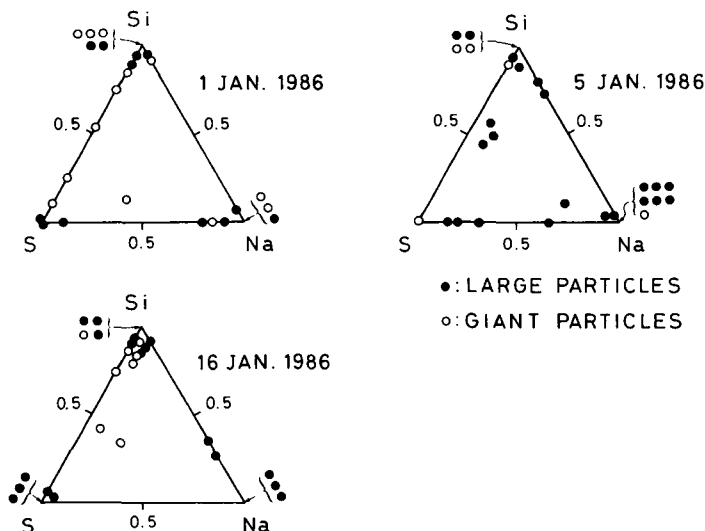
Fig.16. Triangle diagrams of the typical three elements of Si, Na and S of the aerosol particles on each date.
