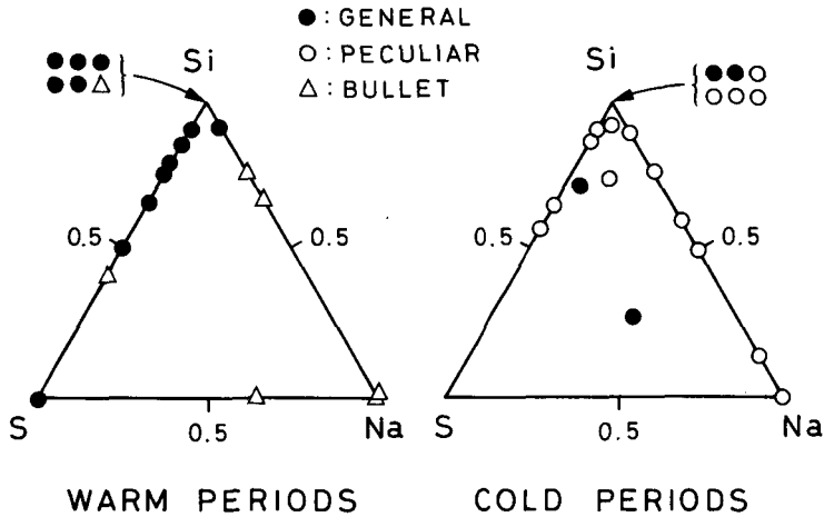
Fig. 19. Triangle diagrams of the typical three elements of Si, Na and S of the center nucleus of snow crystals in the warm and cold periods.
