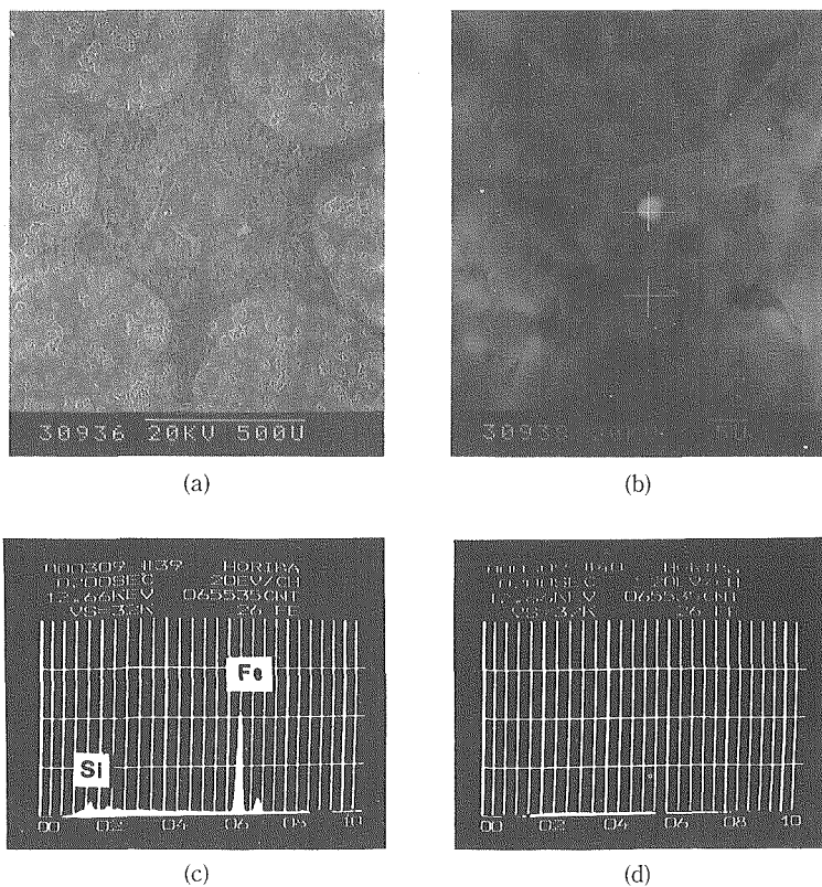
Fig. 3. Analysis of a plate with dendritic extensions. (a) and (b) SEM photographs, (c) and (d) EMAX spectra of the particle and background.
