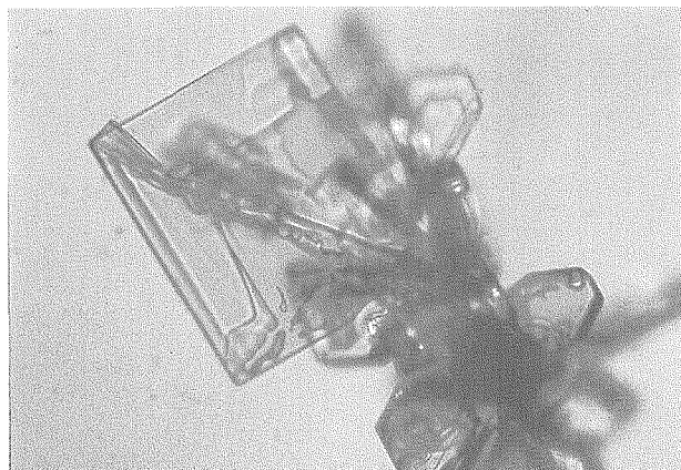
Fig. 6. A microphotograph of snow crystals of low temperature types ( \times 130 ).
