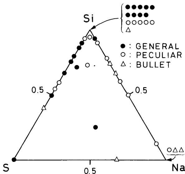
Fig. 11. Triangle diagram of the typical three elements of Si, Na and S of the center nucleus of snow crystals.
