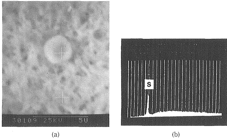
Fig. 15. Same as Fig. 12. (a) SEM photograph, (b) EMAX spectrum.
