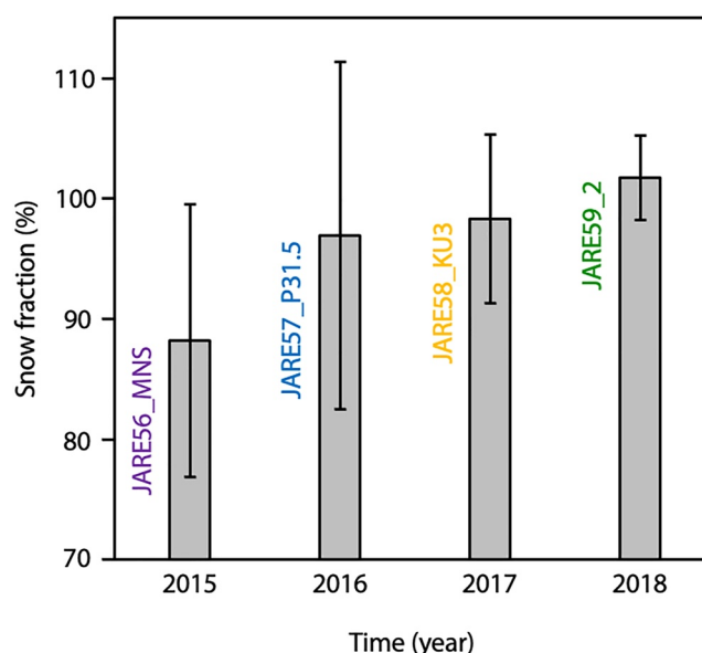
Figure 6. Time series of the mean snow fraction in the top 200 cm of each multi-year ice core from 2015 (core JARE56_MNS) to 2018 (core JARE59_2).
