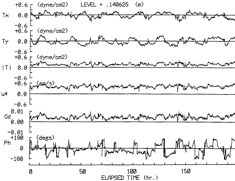
Fig. 9. Estimated time series of near bottom ( z=0.14 m) shear stress components T_x , T_y , magnitude of stress |T| , friction velocity u_* , drag coefficient C_d , and the bearing angle of stress vector P_h against the quasi-geostrophic current vector outside the Ekman boundary layer. The angle P_h is measured with rotating the stress vector by 180^\circ .
