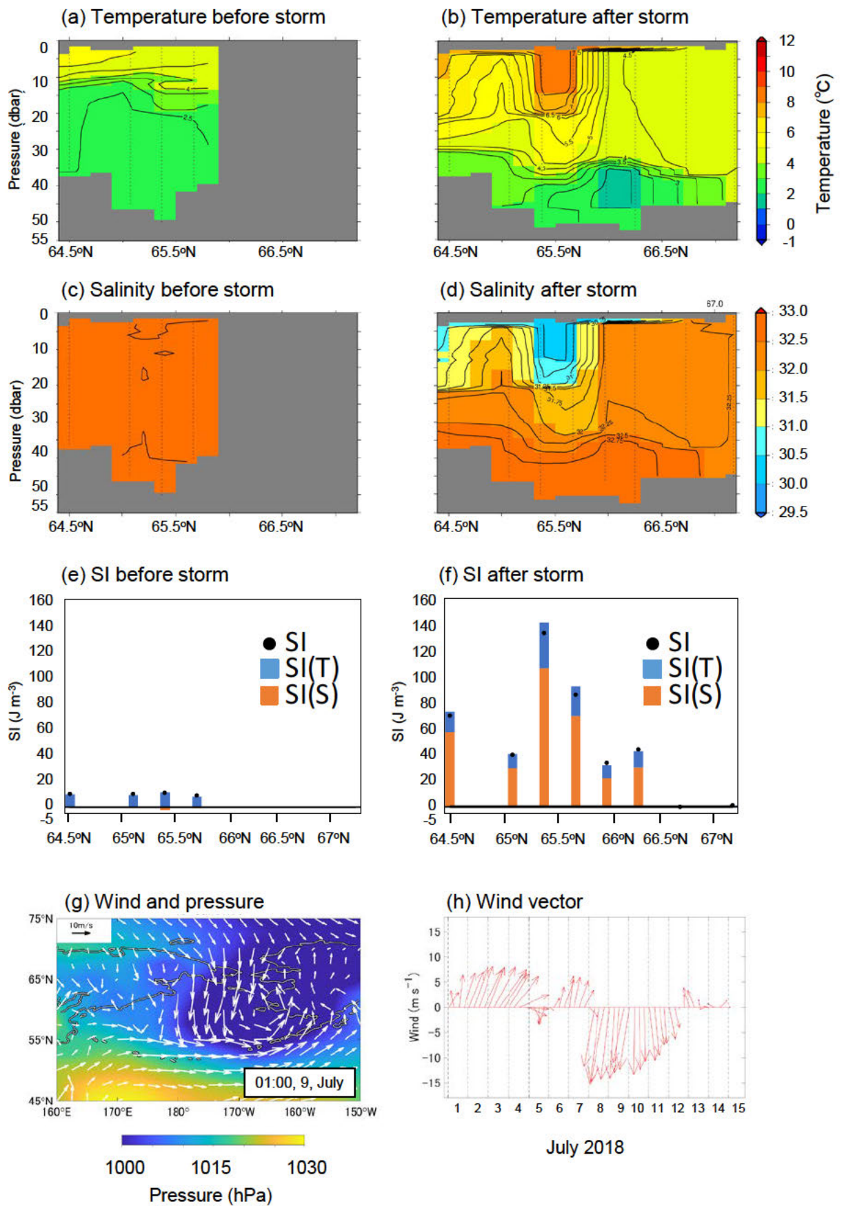
Fig. 7. (a, b) Temperature (°C) and (c, d) salinity cross-sections, and (e, f) SI, SI(S), and SI(T) along ~169°W during July 5–8, 2018 (before passage of low-pressure area (a, c, e)), and during July 10–12, 2018 (after passage of low-pressure area (b, d, f)). Negative SI(S) indicates that the water column is unstable in salinity. (g) Distribution of 10-m wind (vectors, m s -1 ) and surface pressure (color, hPa) at 01:00 (UTC) on July 9, 2018 and (h) time series of 10-m wind vectors over the period July 1–14 2018 at 168.75°W and 66.25°N.
