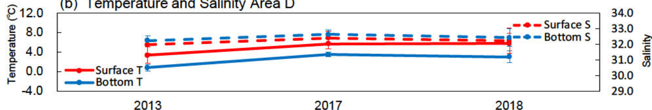
(b) Temperature and Salinity Area D
