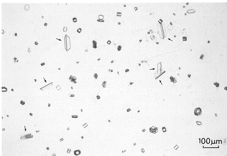
Fig. 3. Microphotograph of ice fog particles taken at Inuvik, Arctic Canada. Arrows indicate poly-snow germs.
