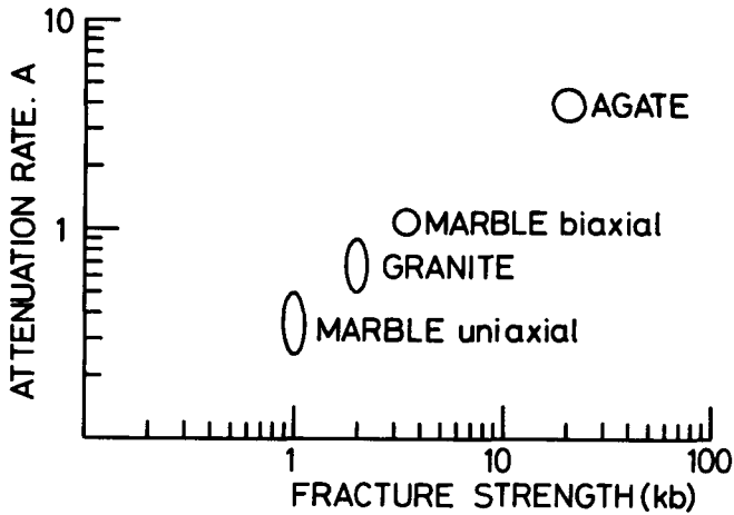
Fig. 4. A log-log plot of attenuation rates, A , of TL versus fracture strengths. The rate, A , is defined by the equation I=1/t^A , where I is TL intensity and t is time.
