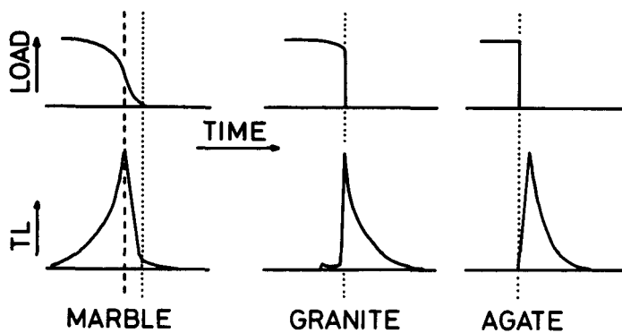
Fig. 3. Patterns of TL and load variations for marble, granite, and agate. Dotted lines indicate the time when the load has returned to zero. Variations of TL are exaggerated around this time.
