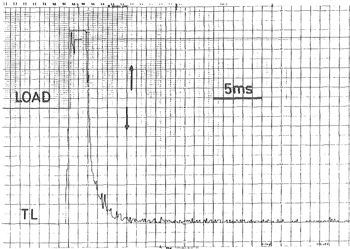
Fig. 1. An example of records of TL and load variations of agate. Upward and downward arrows indicate relative pen positions for the load and TL, respectively.
