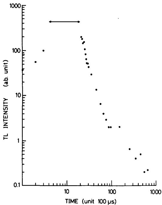
Fig. 2. Variation of TL intensity as a function of time. Data are out-of-scale during the time interval indicated by a horizontal arrow.
