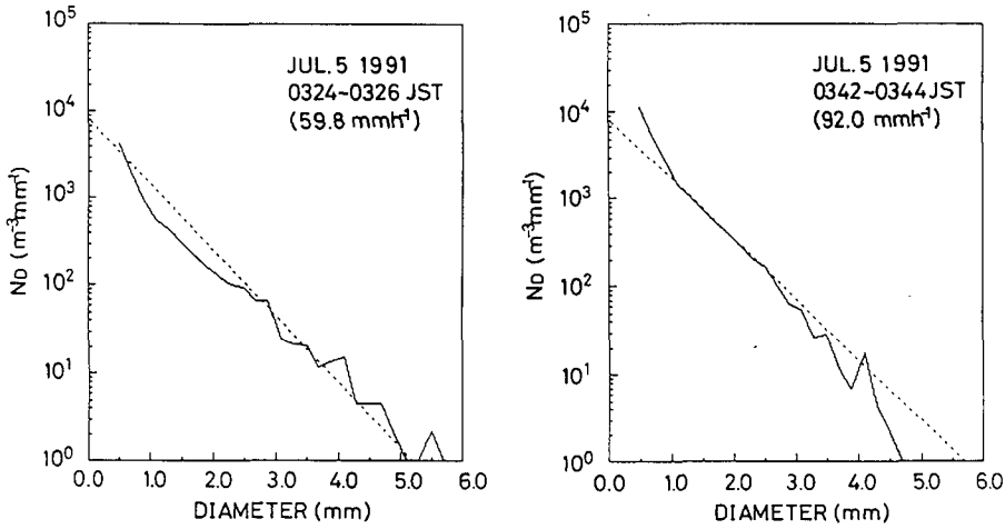
Fig. 16. Rain drop size distributions of the first rainband (left: 0324~0326JST on July 5, 1991) and the second rainband (right: 0342~0344JST).
