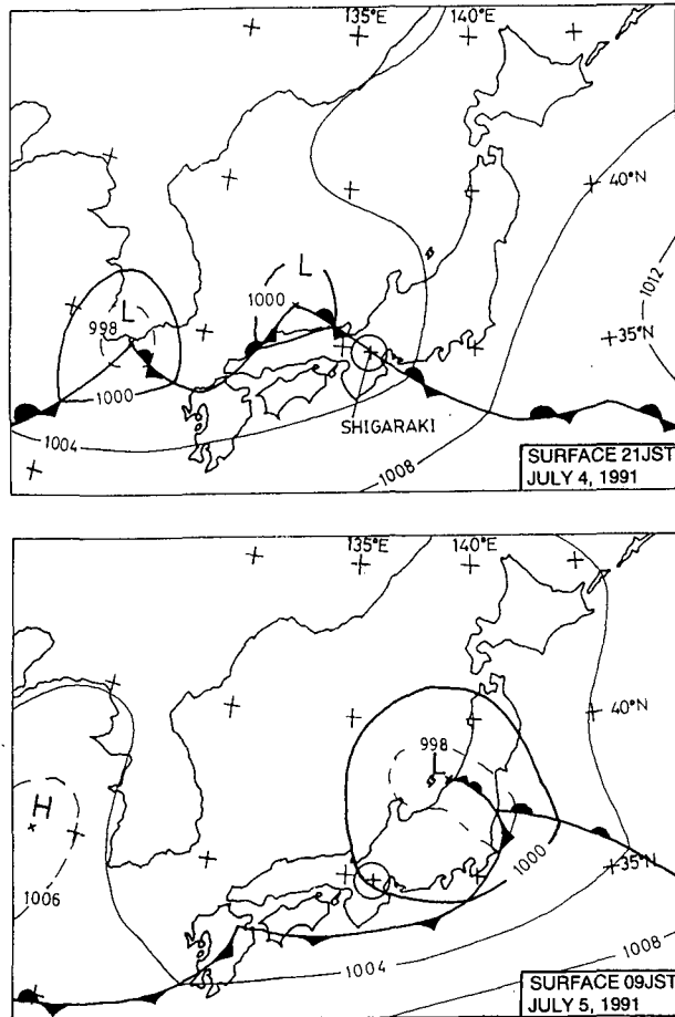
Fig. 2. Surface weather charts at 21JST on July 4 and at 09JST on July 5, 1991. The location of the radar site and its 60 km range is depicted as a cross and a circle, respectively.
