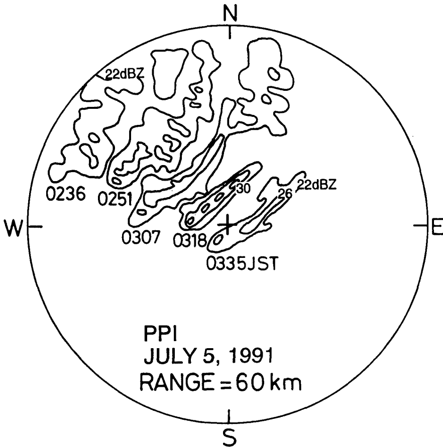
Fig. 7. Transition of PPI scan radar echoes (elevation=4°) from 0236JST to 0335JST on July 5, 1991. Contour interval is 4 dBZ from 22 dBZ.
