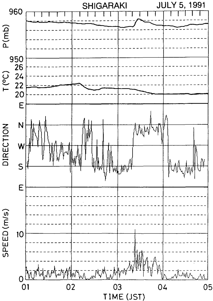
Fig. 11. Surface meteorological observations of transitions in pressure, temperature, and wind from 01JST to 05JST on July 5, 1991, at the radar site.
