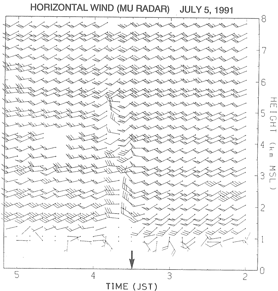
Fig. 4. Wind profiles from 02JST to 05JST on July 5, 1991, obtained by MU radar data. Full barb is a wind speed of 5 \text{ ms}^{-1} , half barb is of 2.5 \text{ ms}^{-1} , and pennant expresses that of 25 \text{ ms}^{-1} .
