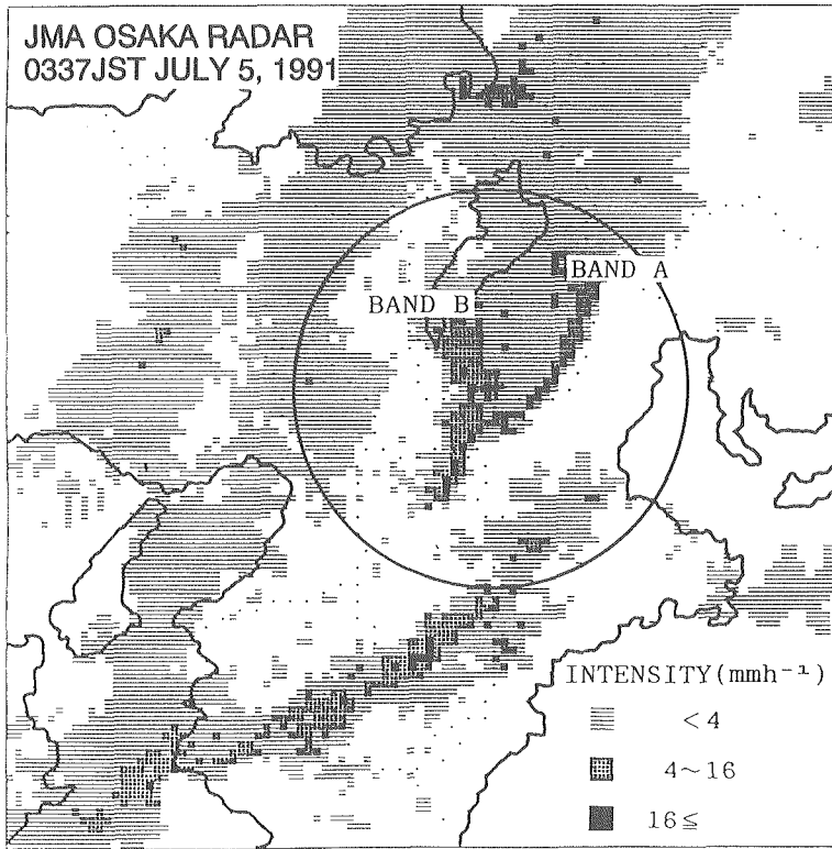
Fig. 5. JMA Osaka radar image around MU radar site at 0337JST on July 5, 1991.
