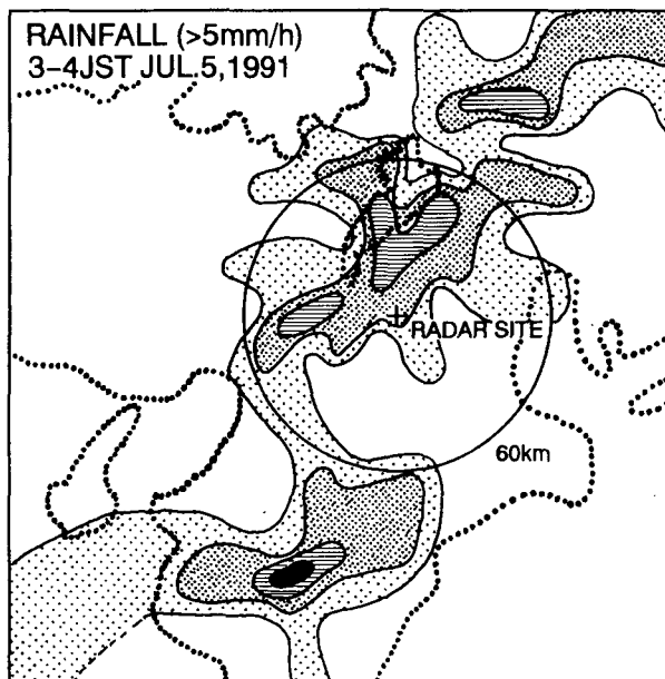
Fig. 12. Distribution of surface rainfall amount from 03JST to 04JST derived from AMeDAS network. Light stippled area expresses rainfall >5 mm, heavy stippled area expresses >10 mm, shaded area expresses >20 mm, and >40 mm area is shaded black. Dotted line indicates the coastal line.
