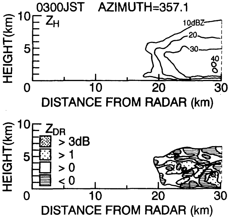
Fig. 9. Vertical cross section (RHI) of the rainband A at the azimuth of 357.1^\circ at 03JST on July 5, 1991. Top: Reflectivity ( Z_H ) in dBZ. Contour interval is 10 dBZ from 10 dBZ. Bottom: Differential reflectivity factor ( Z_{DR} ) in dB.
