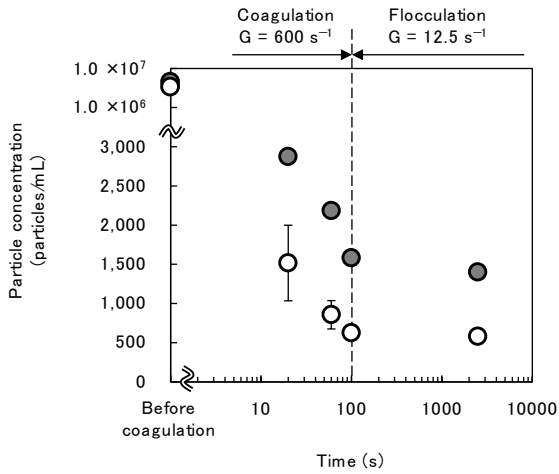
Fig. 9. Change of particle concentration against mixing time during coagulation and flocculation. Batch experiments were conducted using a 1-L rectangular beaker, Municipal water 1 (white plots) or River water 2 (grey plots) as the raw water, and PACI-70 (a) or PACI-50 (b) at 1.5 mg-Al/L as the coagulant. SPAC initial concentration, 2.0 mg/L. Water samples were collected during coagulation and flocculation treatments and then subjected to centrifugal separation treatment (see Section 2.4). Centrifugal supernatants were examined for carbon particle concentration. Water sampled before coagulation was also examined. Two runs were conducted for Municipal water 1, and one run for River water 2. Error bars represent the standard deviations for experiments, but some of them are hidden behind the symbols.
