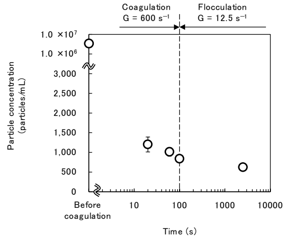
Fig. 9. Change of particle concentration against mixing time during coagulation and flocculation. Batch experiments were conducted using a 1-L rectangular beaker, Municipal water 1 (white plots) or River water 2 (grey plots) as the raw water, and PACI-70 (a) or PACI-50 (b) at 1.5 mg-Al/L as the coagulant. SPAC initial concentration, 2.0 mg/L. Water samples were collected during coagulation and flocculation treatments and then subjected to centrifugal separation treatment (see Section 2.4). Centrifugal supernatants were examined for carbon particle concentration. Water sampled before coagulation was also examined. Two runs were conducted for Municipal water 1, and one run for River water 2. Error bars represent the standard deviations for experiments, but some of them are hidden behind the symbols.
