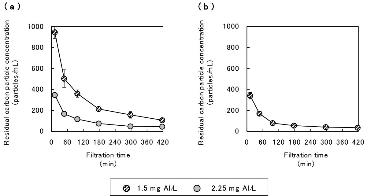
Fig. 2. Residual carbon particle concentration in sand filtrate after treatment of river water (a, River water 1) or municipal water (b, Municipal water 1) with a bench-scale CSF plant. Coagulation: single-chambered reactor, G = 600 \text{ s}^{-1} ; flocculation: 4-chambered reactor, G = 12.5 \text{ s}^{-1} ; filtration rate, 90 \text{ m d}^{-1} . SPAC initial concentration, 2.0 \text{ mg/L} ; coagulant (PACI-70), 1.5 or 2.25 \text{ mg-Al/L} . Error bars indicate standard deviations of 3 measurements, but some of them are hidden behind the symbols.
