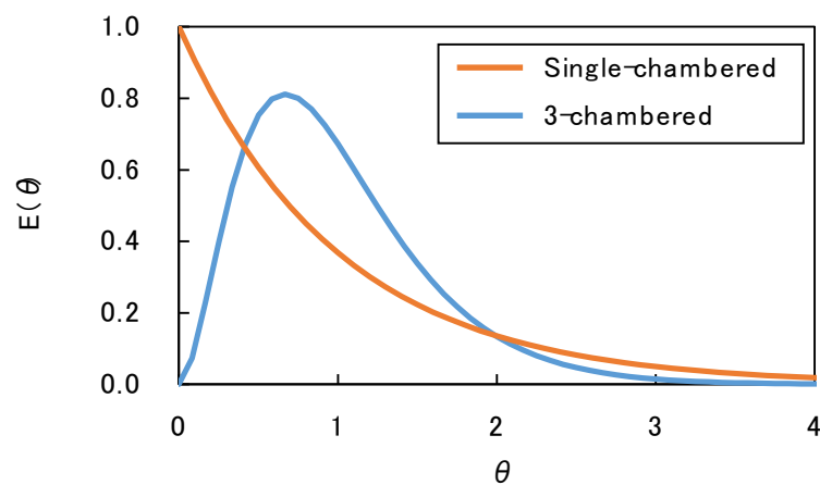
Fig. S6. Theoretical (a) and experimental (b) residence time distributions for the single-chambered or 3-chambered coagulation reactor with rapid mixing. \theta is normalized residence time divided by HRT, and E(\theta) is residence time distribution (Crittenden et al. 2012).
