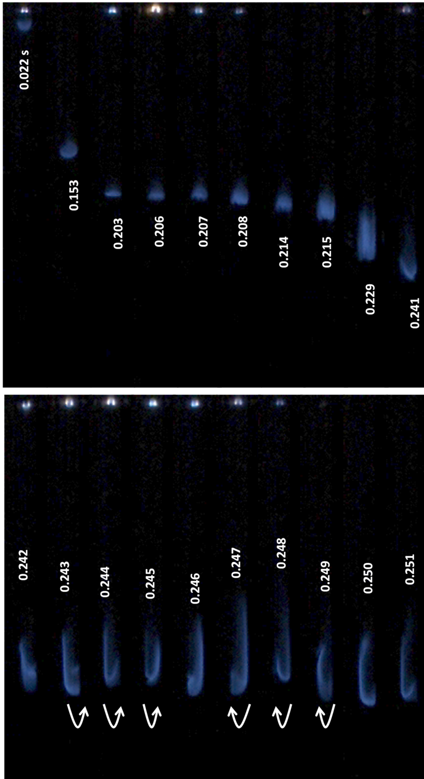
Fig. 14. Flame images at various instances showing corrugations on the flame front during parametric instability of first harmonic and rotating flame front during regime VI-N at S_L=35.0 cm/s Top 18.5 cm of the tube is shown. Time in seconds from ignition is also noted.
