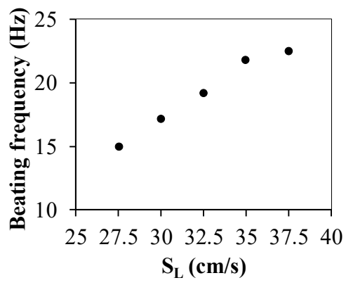
Fig.12. Beating frequency at various S_L .
