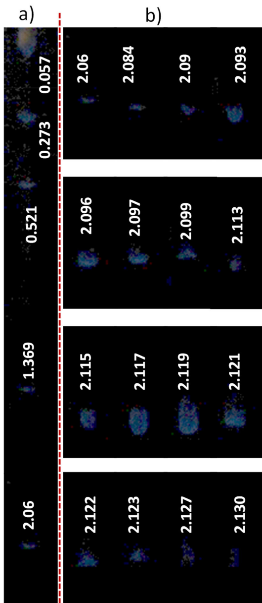
Fig. 5. Flame images at various times during regime IV-N, S_L = 15.0 cm/s a) shows top 20 cm of the tube b) shows 15.5 cm to 20 cm from top where flame extinction occurs. The numbers indicate time in seconds from the ignition.
