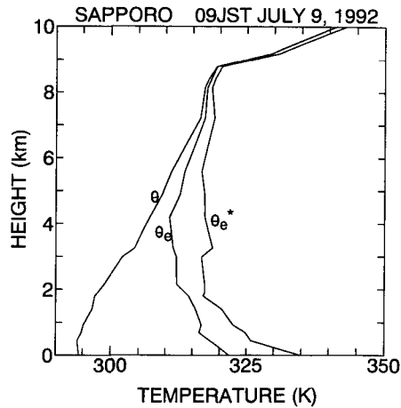
Fig. 3. Vertical profiles of potential temperature, equivalent potential temperature, and saturated equivalent potential temperature at 09JST on July 9, 1992.
