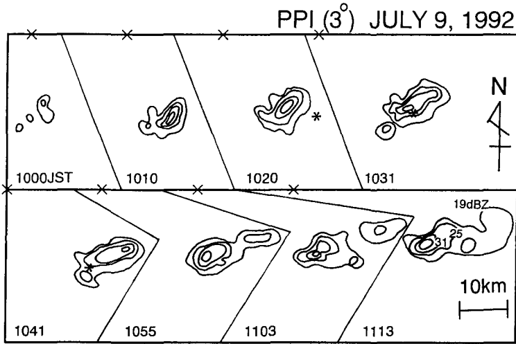
Fig. 4. Transition of PPI scan radar echoes (elevation = 3^\circ ) from 1000JST to 1113JST on July 9, 1992. Contour interval is 6 dB from 19 dBZ. The symbol ( \times ) indicates the relative position of the radar site. Also, the locations of Eniwa-Shimamatsu relative to the echo at 1020JST, 1031JST, and 1041JST are indicated by the symbol (*).
