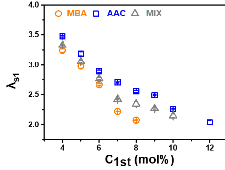
Figure S5. The length swelling ratio \lambda_{S1} of the three sets of PAMPS SN gels in the AAm monomer solution, which is determined by the thickness of the equilibrated PAMPS SN gels in AAm monomer solution divided by the thickness of the as-prepared PAMPS SN gels.
