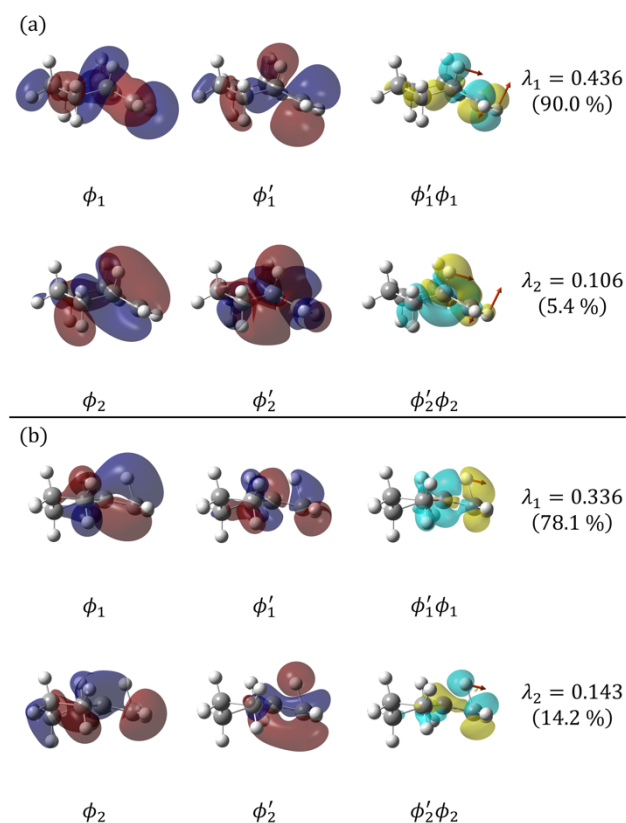
Figure 20. NRO pairs of the maximum singular value ( \phi_1 and \phi'_1 ) and the second maximum singular value ( \phi_2 and \phi'_2 ), which are calculated (a) at the TS structure and (b) at the point X in Fig. 19 for carbocation rearrangement. The products of the NRO pairs are shown with the tangent vectors of the IRC.
