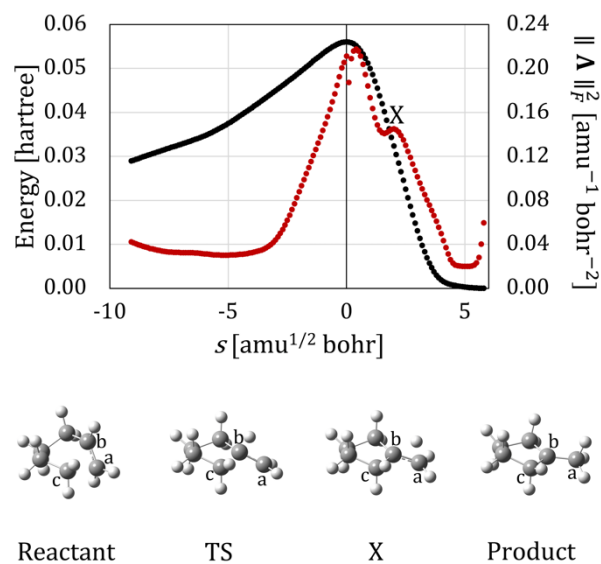
Figure 19. Potential energy profile (black dots) and \|\mathbf{A}\|_F^2 (red dots) for the IRC of the carbocation rearrangement reaction of cyclohexyl cation to methylcyclopentyl cation. The structures at the reactant, TS, X, and product are also shown below.
