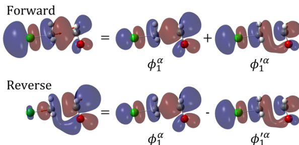
Figure 6. Orbital mixing of occupied and virtual NRO pairs ( \phi_1^\alpha and \phi_1'^\alpha ) with the maximum singular value for nuclear displacements in the directions toward the product (forward) and the reactant (reverse) along the imaginary frequency mode at the ET-TS of the \text{H}_2\text{CO}^- + \text{CH}_3\text{Cl} reaction.
