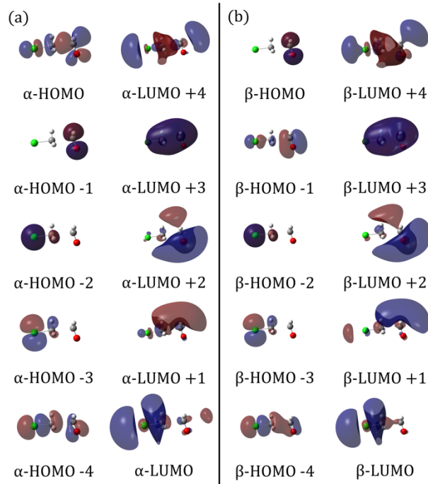
Figure 2. Five occupied and five virtual valence CMOs at the ET-TS for (a) \alpha - and (b) \beta -spin electrons with the isovalue of 0.02.
