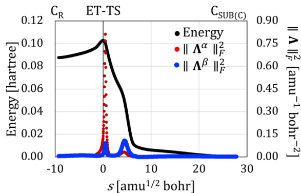
Figure 8. Potential energy along the IRC of the \text{H}_2\text{CO}^- + \text{CH}_3\text{Cl} reaction, for which the energy of the product, C_{\text{SUB}(\text{C})} , is set to be zero, and the \|\Lambda^\alpha\|_F^2 and \|\Lambda^\beta\|_F^2 values. The first peak of \|\Lambda^\alpha\|_F^2 near the ET-TS structure ( 0.47 \text{ amu}^{1/2} \text{ bohr} ) mainly corresponds to the \alpha -NRO pair of Fig. 3 and the second peak of \|\Lambda^\beta\|_F^2 at the shoulder of the potential energy ( 4.49 \text{ amu}^{1/2} \text{ bohr} ) corresponds to the \beta -NRO pair.
