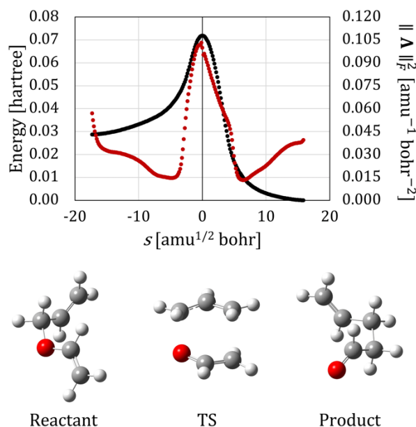
Figure 10. Potential energy profile (black dots) and \|\mathbf{A}\|_F^2 (red dots) for the IRC of the Claisen rearrangement reaction of \text{C}_3\text{H}_5\text{OC}_2\text{H}_3 molecule, for which the product energy is set to be zero. The molecular structures of the reactant, TS, and product are also shown below.
