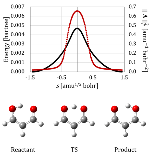
Figure 15. Potential energy profile (black dots) and \|\Lambda\|_F^2 (red dots) for the IRC of the intramolecular proton transfer in malonaldehyde. The structures at the reactant ( C_s ), TS ( C_{2v} ), and product ( C_s ) are also shown below.
