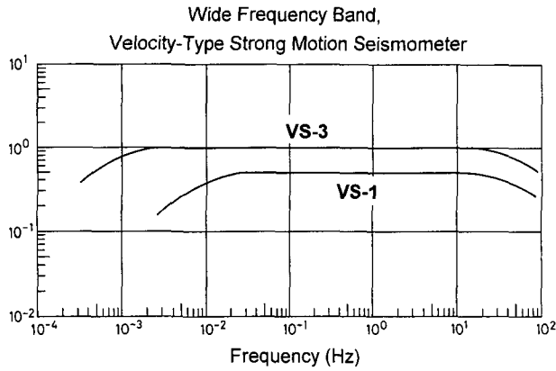
Fig. 6. Frequency characteristics of the velocity-type strong motion seismometers, VS-1 and VS-3 (Muramatu, 1995).
