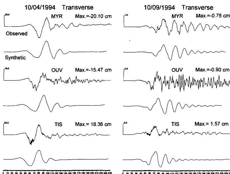
Fig. 11. Comparison between the observed and synthetic seismograms (transverse component) for the main shock (left) and the largest aftershock (right) at MYR, OUV and TIS. The synthetic seismograms are calculated for the estimated source parameters shown in Table 3.
