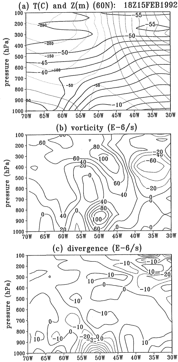
Fig. 4. Vertical cross sections along 60^{\circ}N at 1800 UTC, 15 February 1992 of (a) height deviation from the averaged height between 30^{\circ}W and 70^{\circ}W (thin lines in meter) and temperature (thick lines in ^{\circ}C ), (b) vorticity ( 10^{-6} s^{-1} ), and (c) divergence ( 10^{-6} s^{-1} ).
